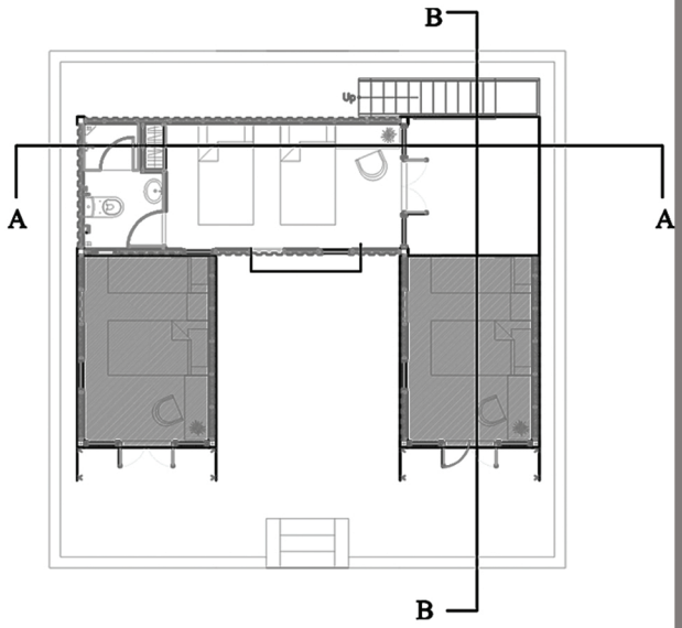
02 FIRST FLOOR PLAN
