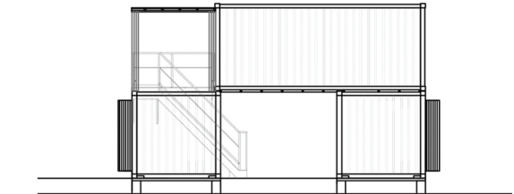
03 BACK ELEVATION
