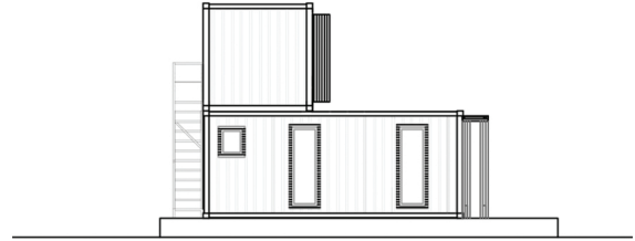
05 LEFT ELEVATION
