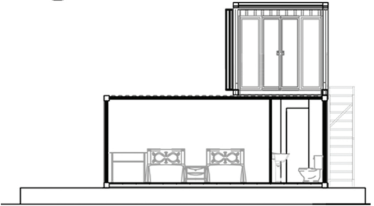
07 SECTION AA
