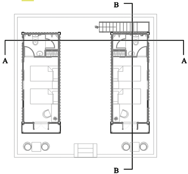
01 GROUND FLOOR
