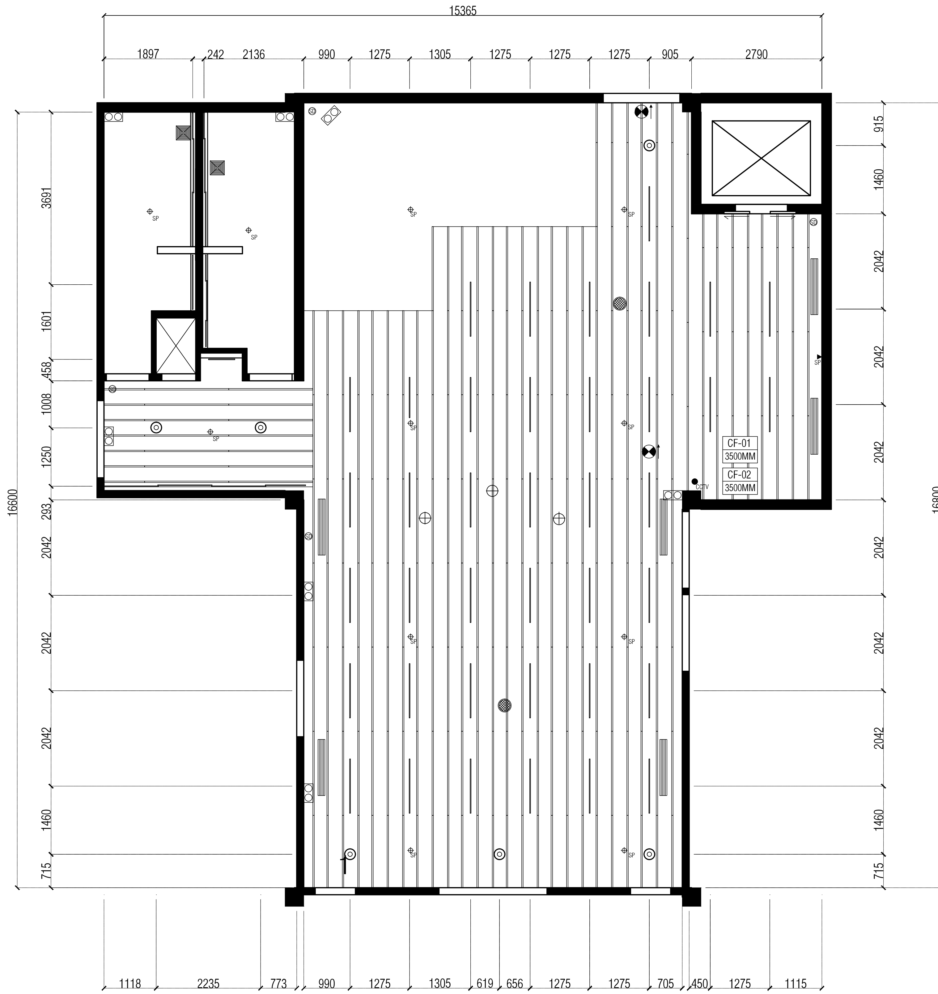
1 AREA 1: RECEPTION AREA REFLECTED CEILING PLAN ID - 01 SCALE 1:50 MTRS
