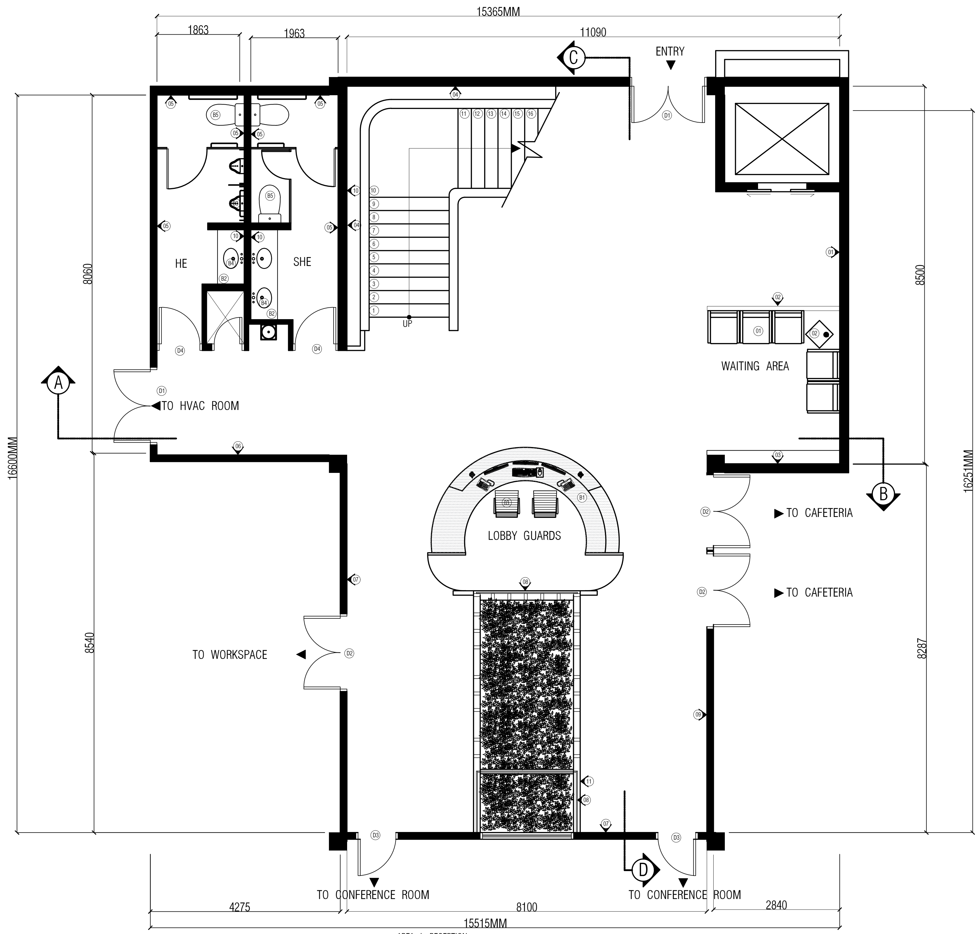
1 ID - 02 AREA 1: RECEPTION FLOOR PLAN W/ FURNITURE LAYOUT SCALE 1:50 MTRS
