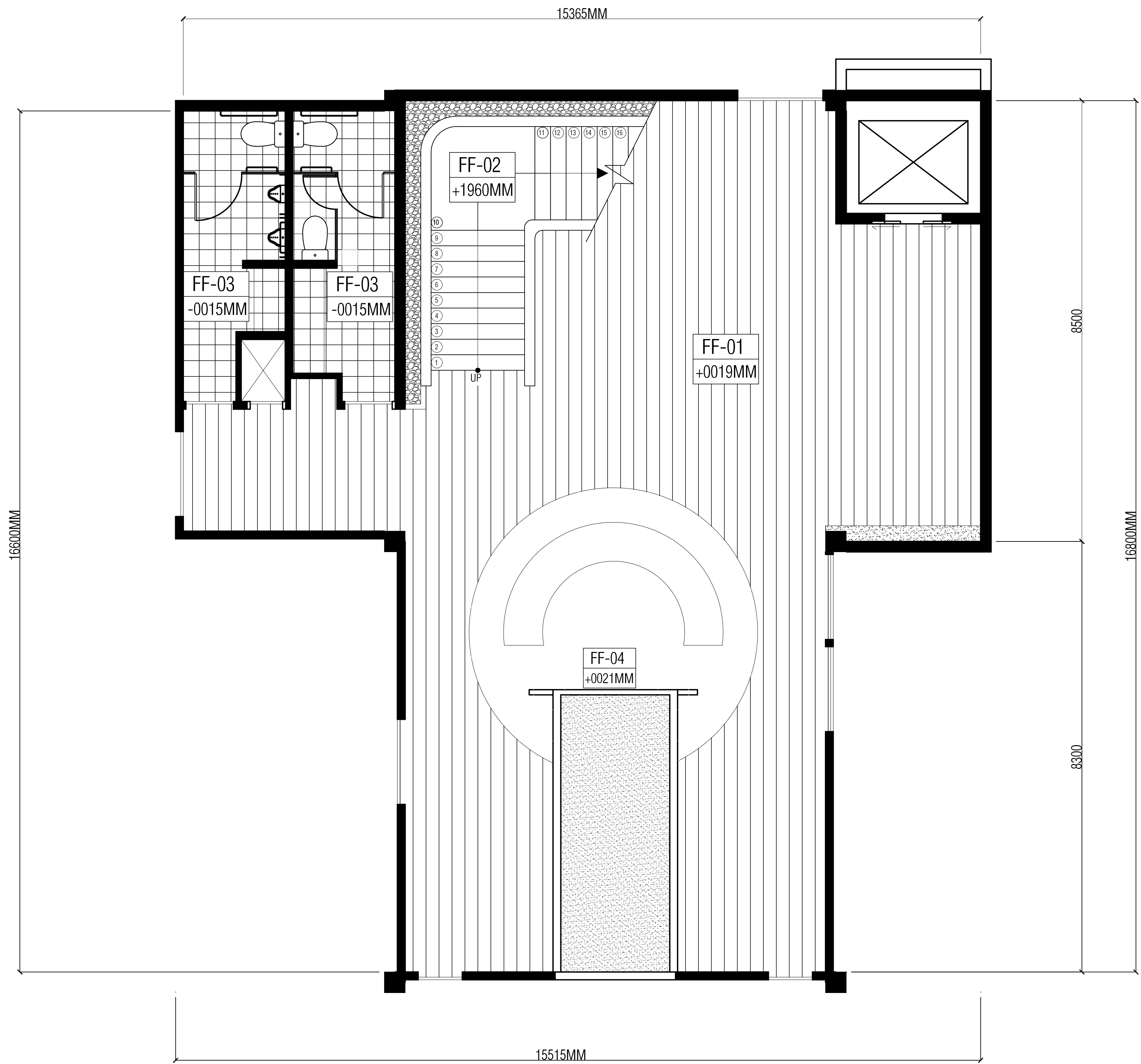
1 AREA 1: RECEPTION FLOOR PLAN W/ FLOOR PATTERN LAYOUT ID - 03 SCALE 1:50 MTRS
