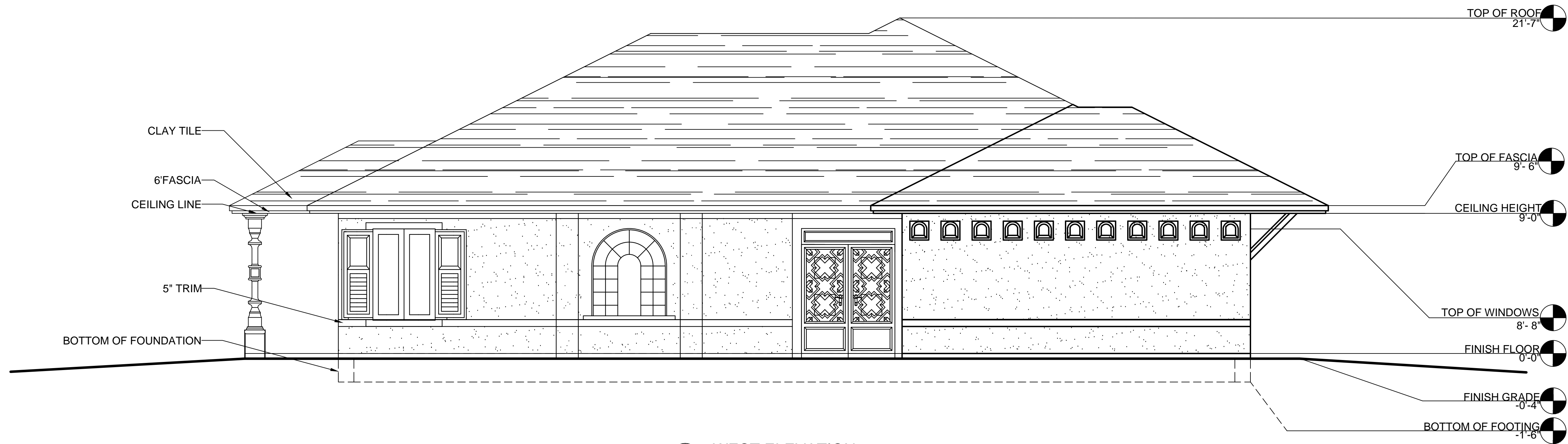
WEST ELEVATION 1/4" = 1'-0"
