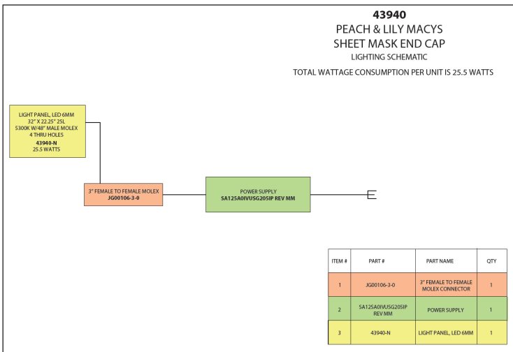
lighting schematic
