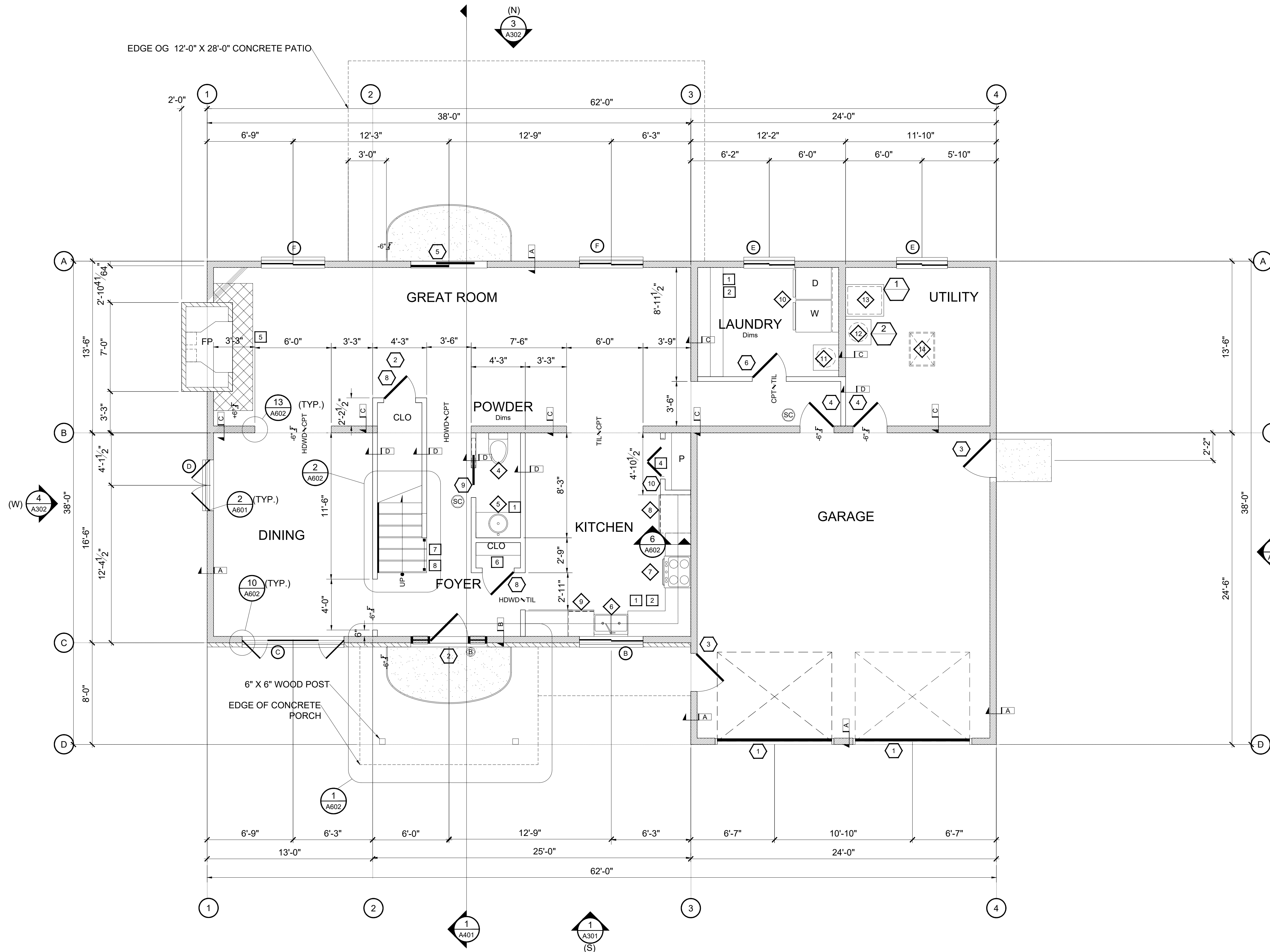
FIRST FLOOR PLAN 1 1/4"=1'-0"
