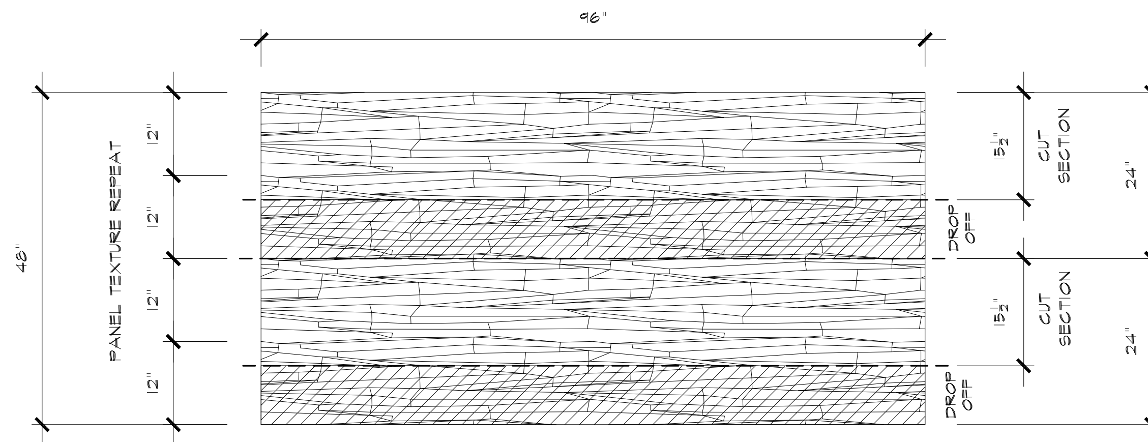
PANEL CUT INSTRUCTIONS \frac{1}{2}'' = 1'-0''
