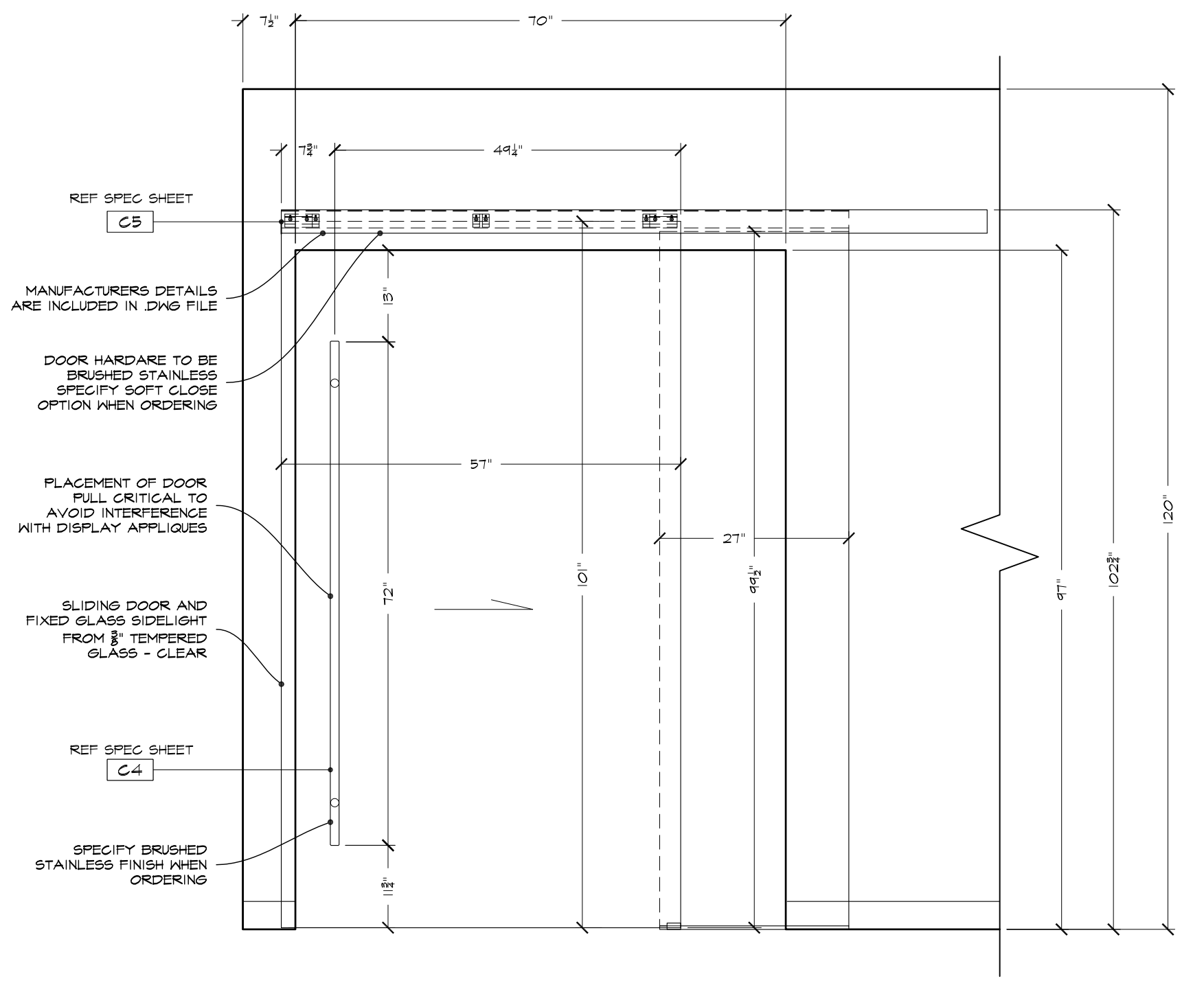
01 S1.2 DETAIL - SLIDING GLASS DOOR
