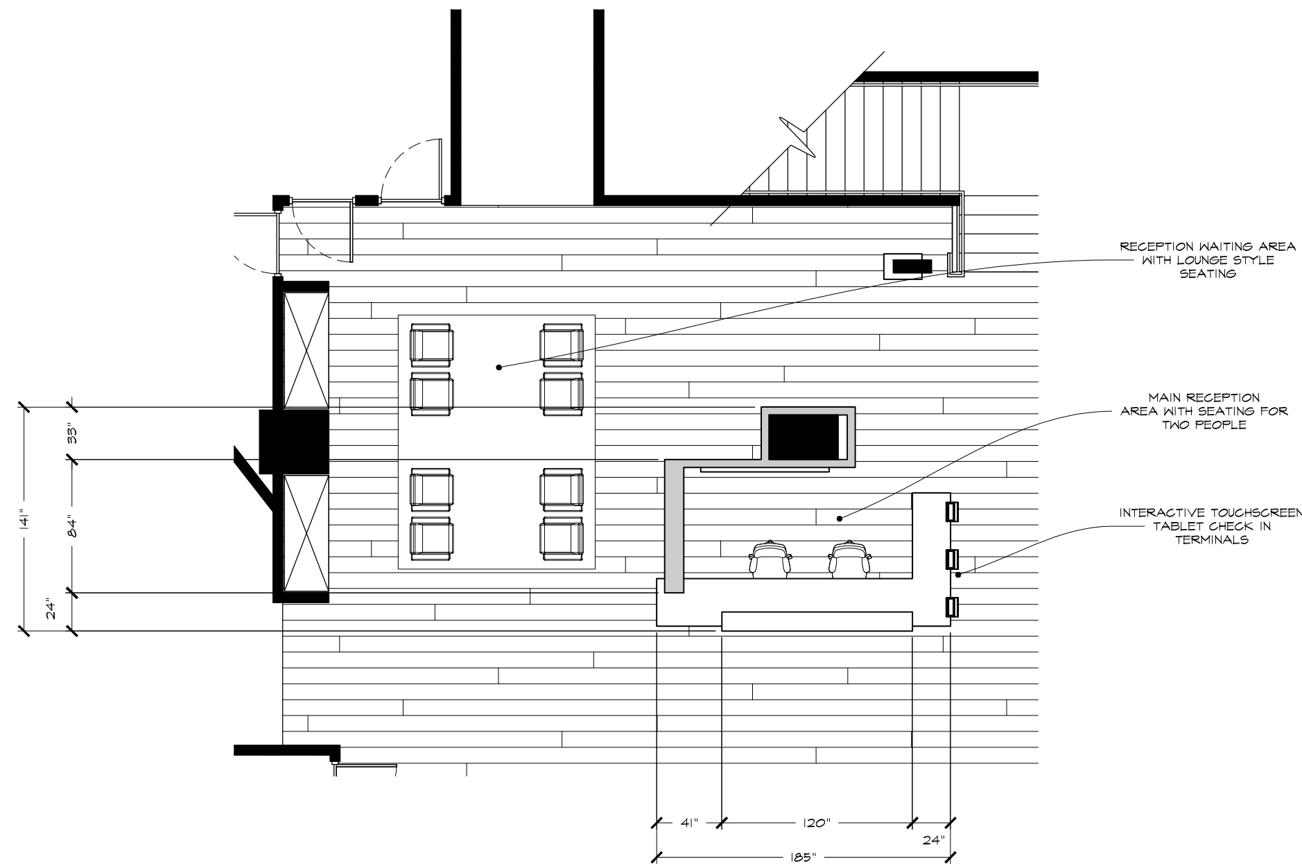
1 LEVEL 1 - RECEPTION AREA SCALE: 3/16" = 1'
