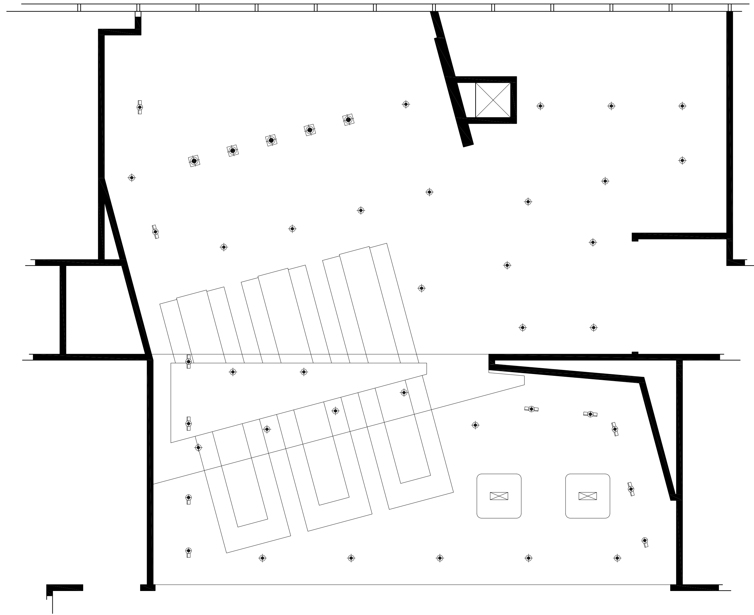
RCP LIGHTING SCHEMATIC LOBBY/COMMON AREAS SCALE: 3/16"=1'-0"
