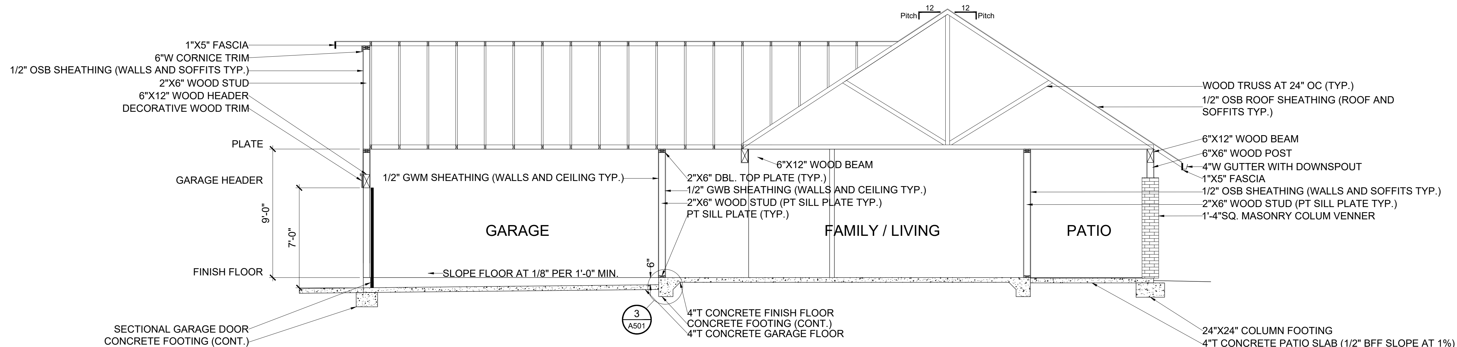
BUILDING SECTION SCALE 1/4"=1'-0"
