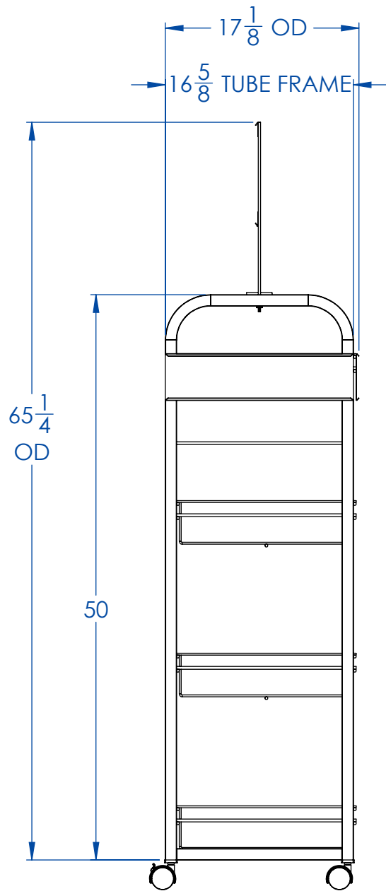
SIDE VIEW
