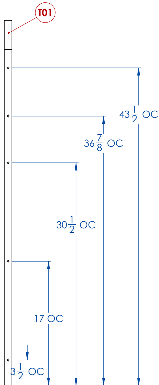
SIDE VIEW - SIDE U TUBE
