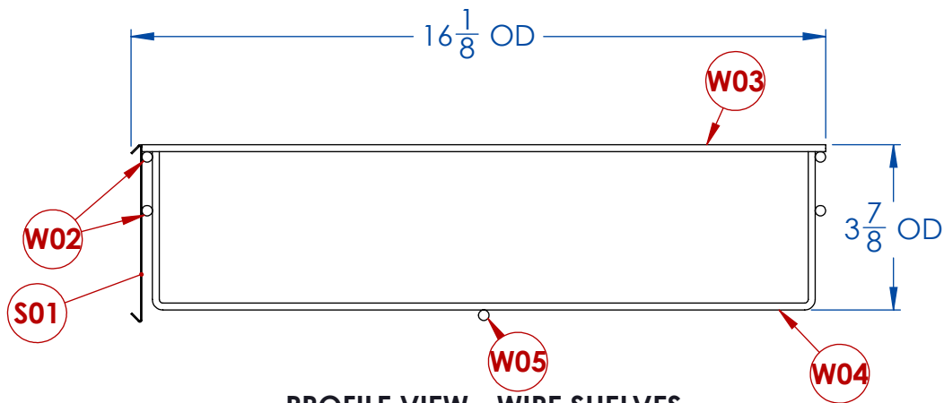
PROFILE VIEW - WIRE SHELVES
