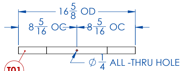
TOP VIEW - SIDE U TUBE
