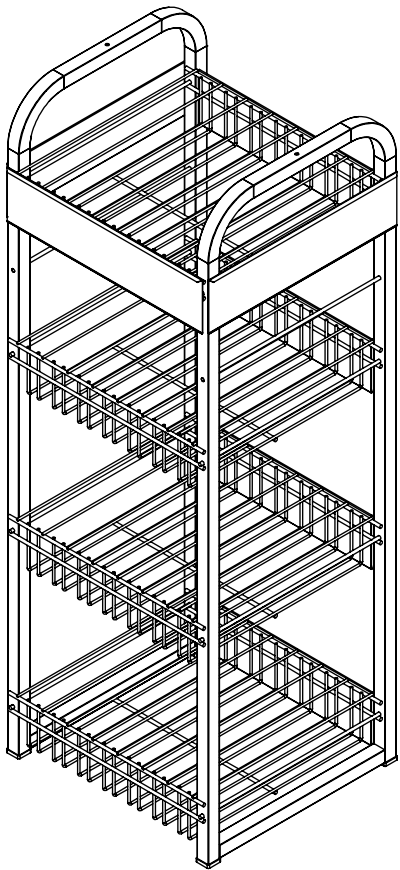
ISOMETRIC VIEW - BACK LEFT
