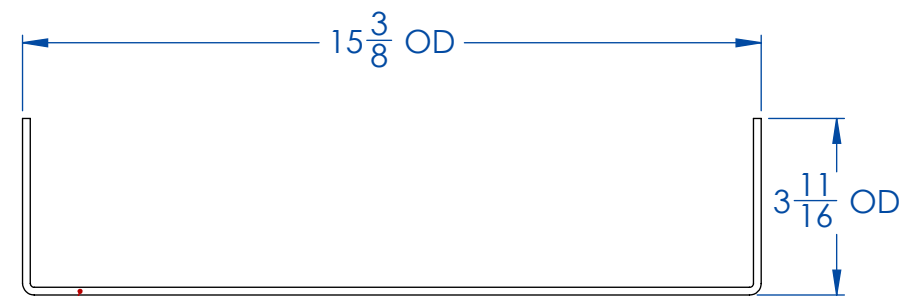
PROFILE VIEW - W04 SHELF U WIRE
