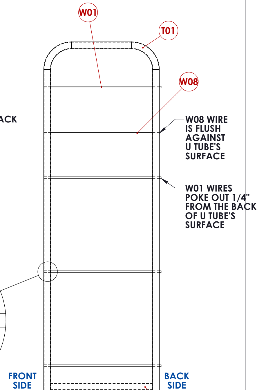
FRONT VIEW - U TUBE ASSEMBLY
