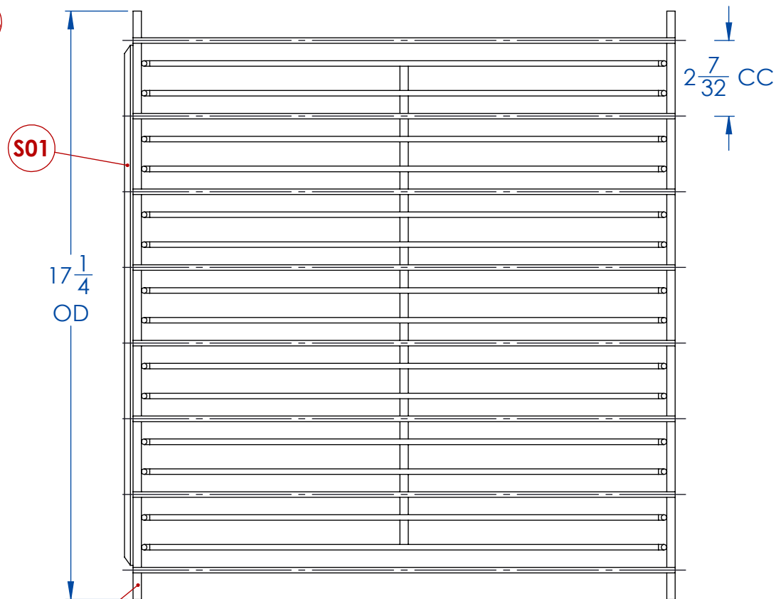
TOP VIEW - WIRE SHELVES
