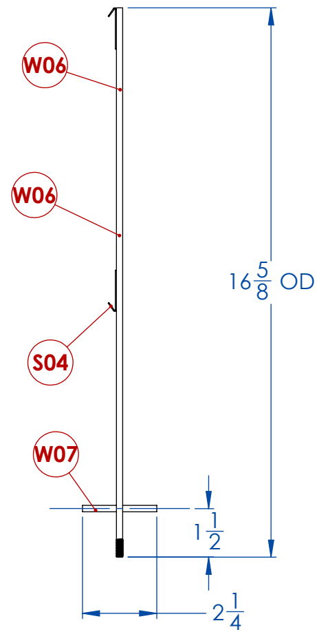
SIDE VIEW - REMOVABLE PTM ASSEMBLY
