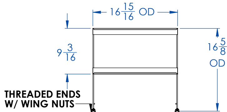
FRONT VIEW - HEADER ASSEMBLY
