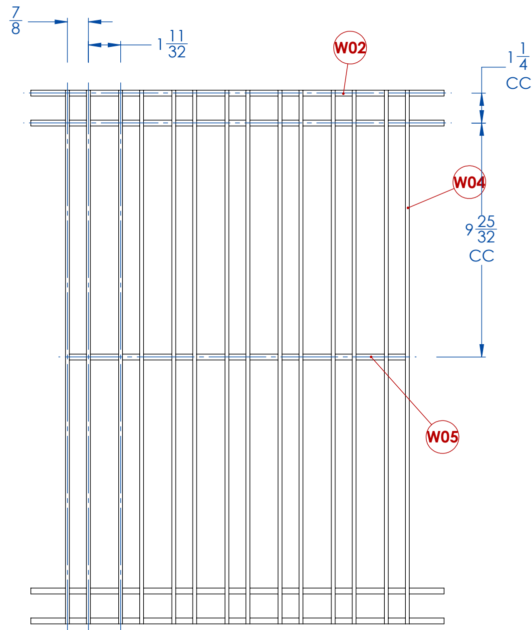
FLAT VIEW - WIRE SHELVES
