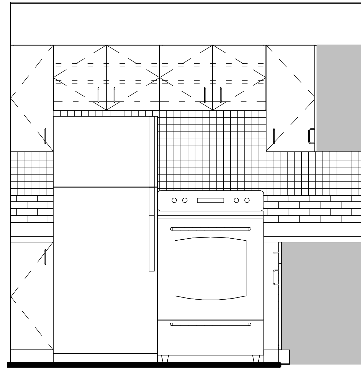
KITCHEN ELEVATION
