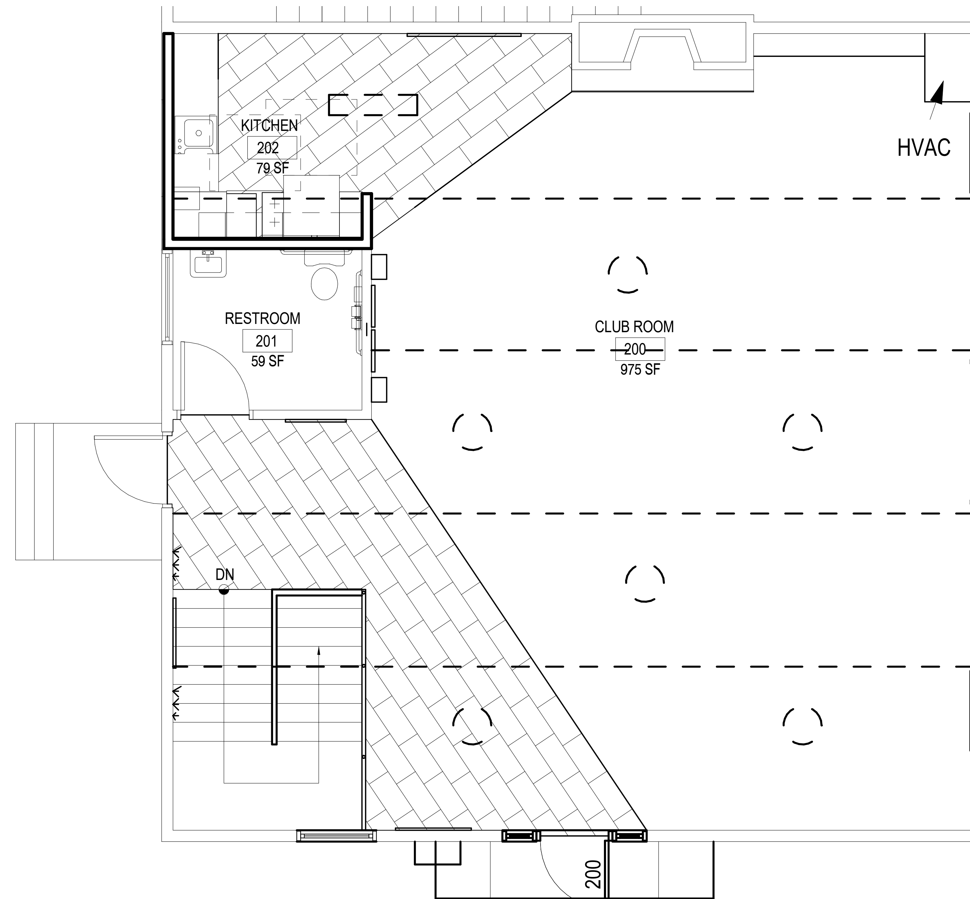
LIGHTING PLAN
