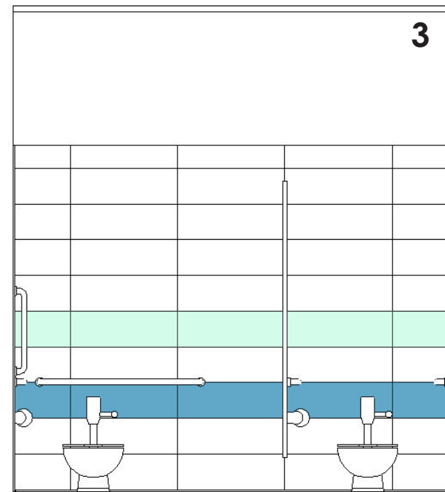
Boys Toilet Elevation
