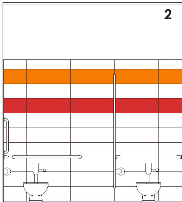
Girls Toilet Elevation
