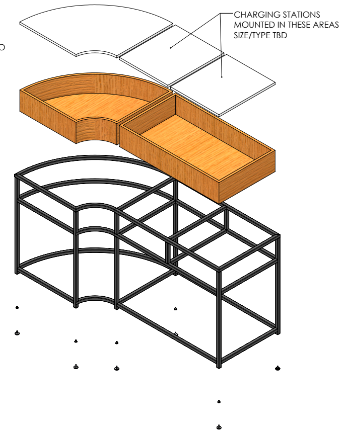
RETAIL TABLE W/ CHARGING STATION:
