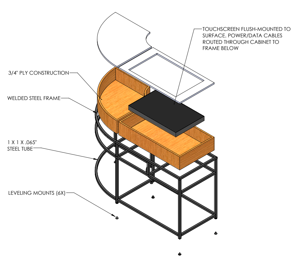
RETAIL TABLE W/ TOUCHSCREEN:
