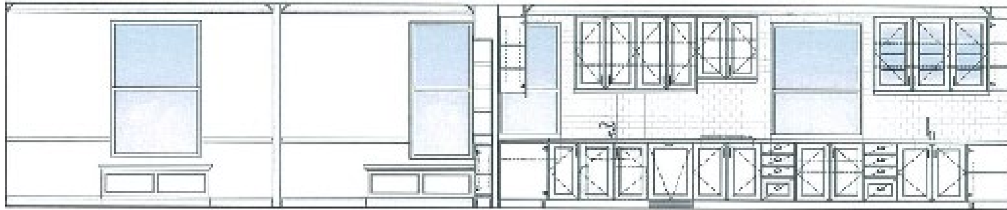
MASTER BEDROOM/ GUEST BEDROOM/ KITCHEN NORTH SECTION/ELEVATION
