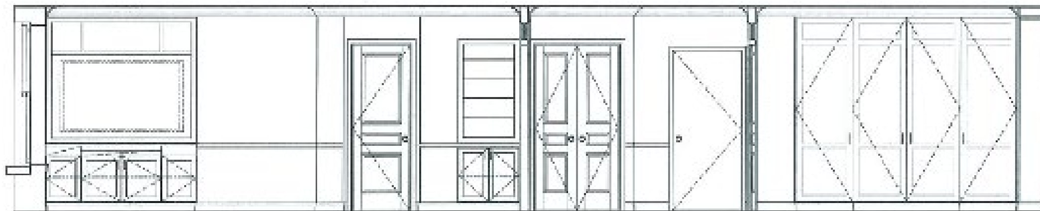
LIVING ROOM/HALL/MASTER CLOSET SOUTH SECTION/ELEVATION
