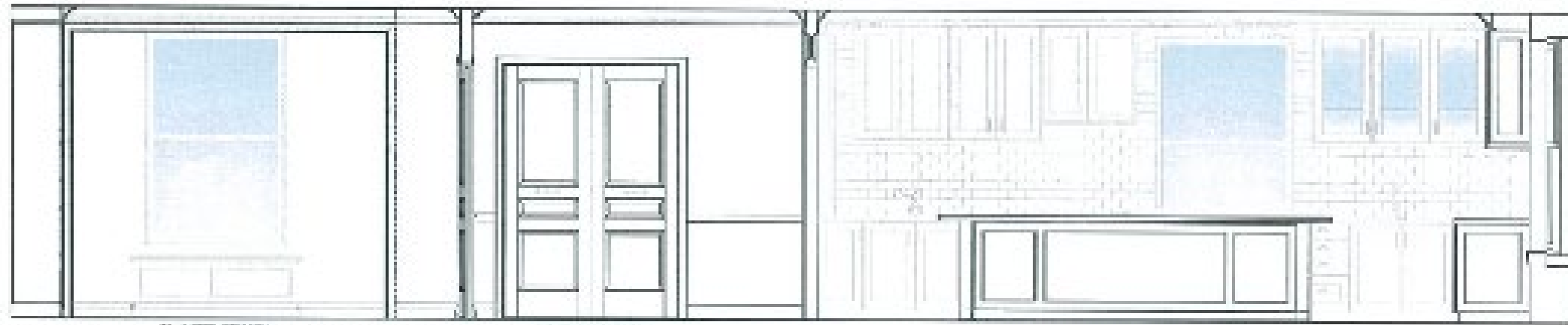
MASTER BEDROOM/HALL/KITCHEN NORTH SECTION/ELEVATION
