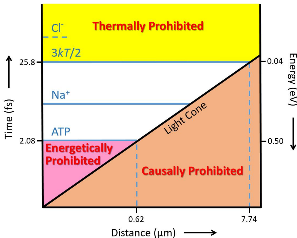
Figure 1. Minimal switching times for transition to an orthogonal state are determined by the energy of quantum entities. Time-energy-distance scales are shown for biologically-relevant processes. The permitted zone is in white. States could persist for longer times if isolated from the surrounding heat bath, but shorter times are excluded by the Margolus-Levitin Theorem [1998], which sets the minimum time required for a quantum entity to switch between orthogonal states, t \geq h/4E .
