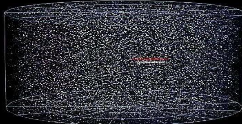
Observable Universe
