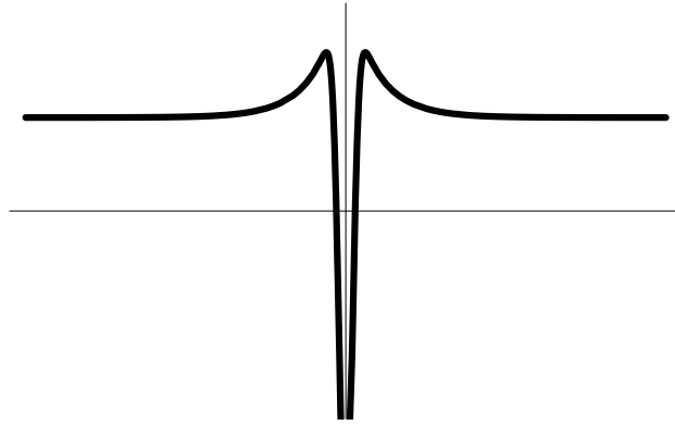
Figure 5. Potential for the graviton modes in a de Sitter brane
