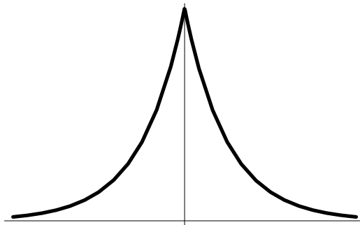
Figure 1. Warping factor a(y) .
