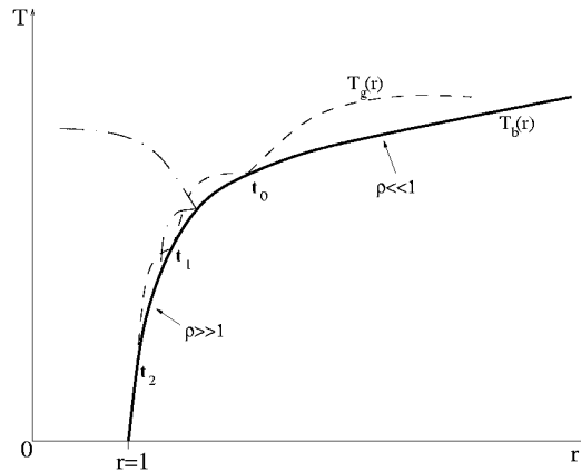
Figure 3. Examples of graviton trajectories in the bulk (dashed line). The brane trajectory, with relativistic matter, is also shown (continuous line).
