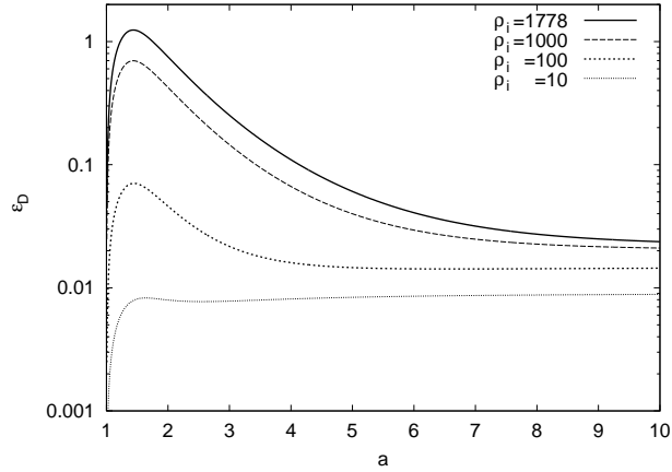
Figure 4. Evolution of the ratio \epsilon_D = \rho_D/\rho for different values of the initial energy density on the brane \rho_i (in units of \sigma^4 ).
