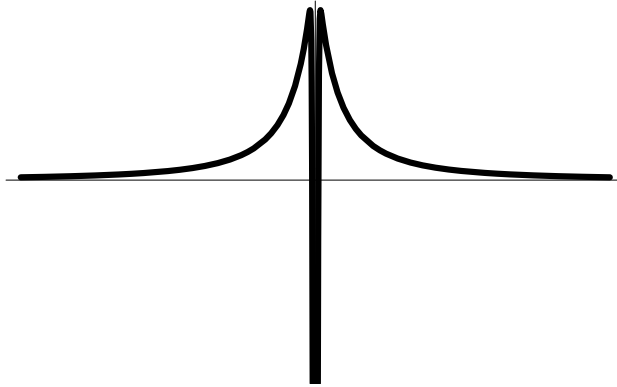
Figure 2. Effective potential of the Schrödinger-like equation that governs the dependence on the fifth dimension.
