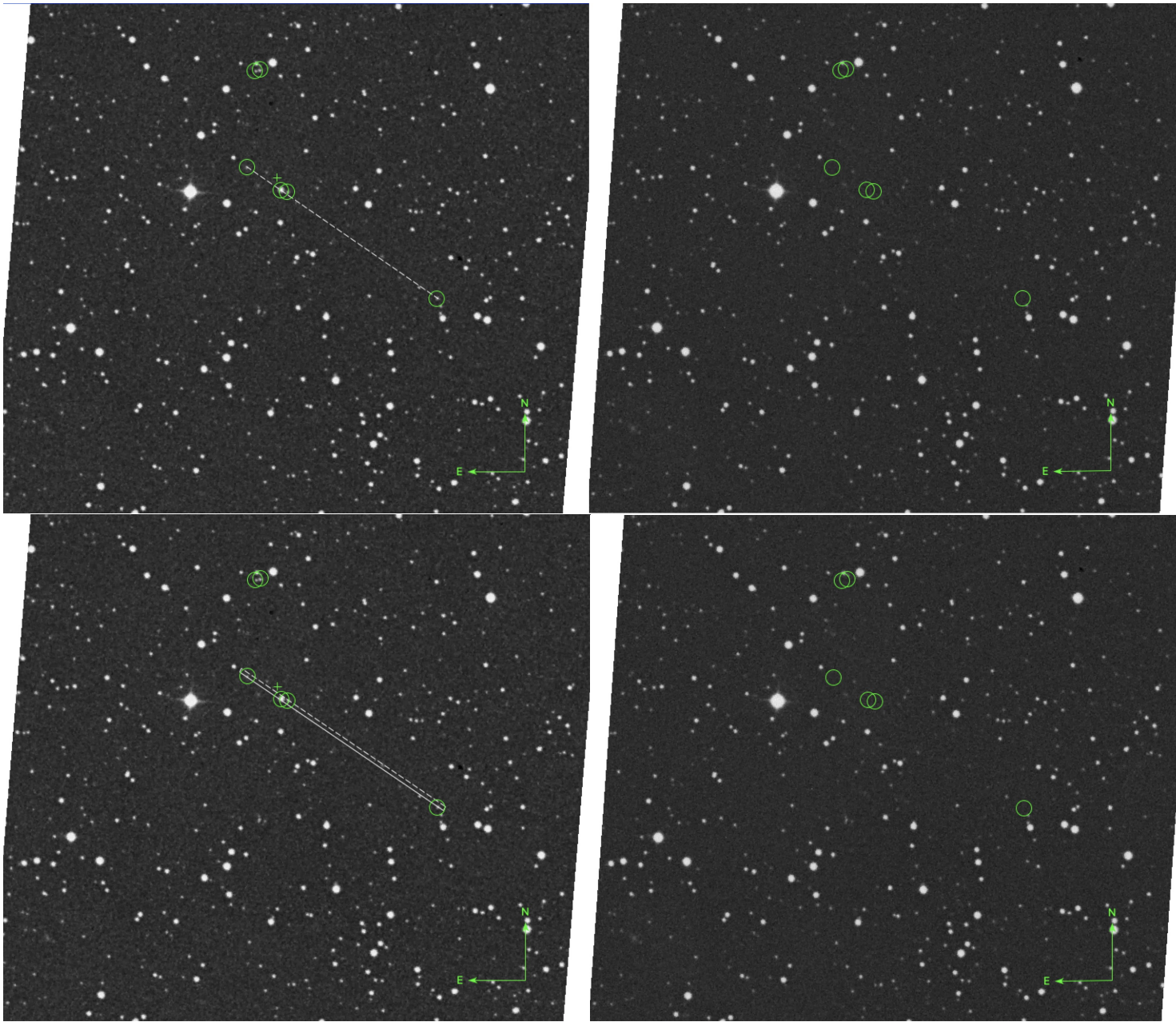
Figure 11. Candidate 4. We show the candidate in SuperCosmos scans of POSS-I red (left) and POSS-II red (right) images. The upper row shows a 3-point alignment within 1 arcsec. The lower row shows a 4-point alignment of within 5 arcsec. Transients are marked with green circles. The candidate with a measured coordinate is marked with a cross (+). The dashed lines shows the alignment (the white double line for the thicker alignment below).
