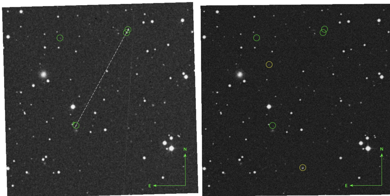
Figure 8. Candidate 1. We show the candidate in SuperCosmos scans of POSS-I red (left) and POSS-II red (right) images. Transients are marked with green circles. The candidate with a measured coordinate is marked with a cross (+). A dashed white line shows the alignment. Yellow circles show defects. Also the white line crossing the POSS-I field is a scanning defect. We see 4 transients in the POSS-I images where three follow a straight line.
