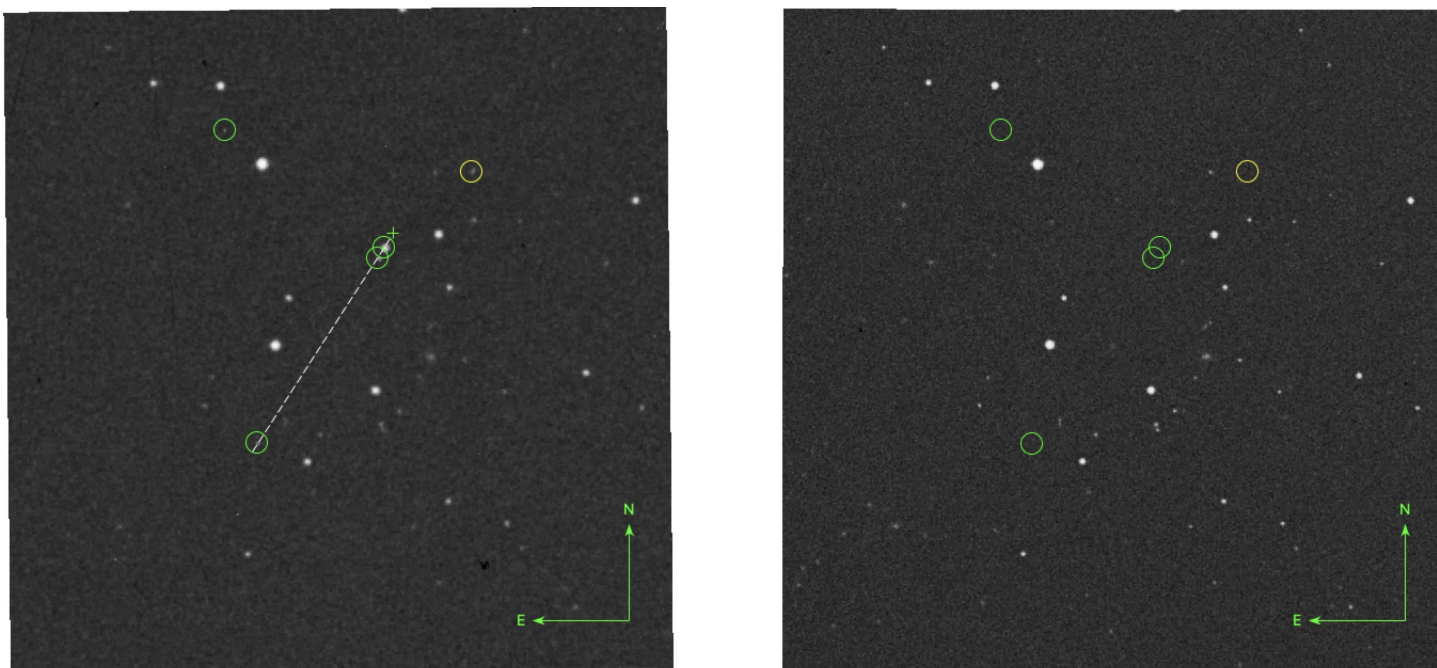
Figure 9. Candidate 2. We show the candidate in SuperCosmos scans of POSS-I red (left) and POSS-II red (right) images. Transients are marked with green circles. The candidate with a measured coordinate is marked with a cross (+). A dashed white line shows the alignment. Yellow circles show defects. Also the white line crossing the POSS-I field is a scanning defect. We see 4 transients in the POSS-I images where three follow a straight line.
