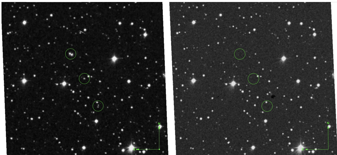
Figure 6. Red vs. blue image of Candidate 5. Comparison between the red (left) and blue (right) DSS images for Candidate 5. No coincident sources are found in the blue image.
