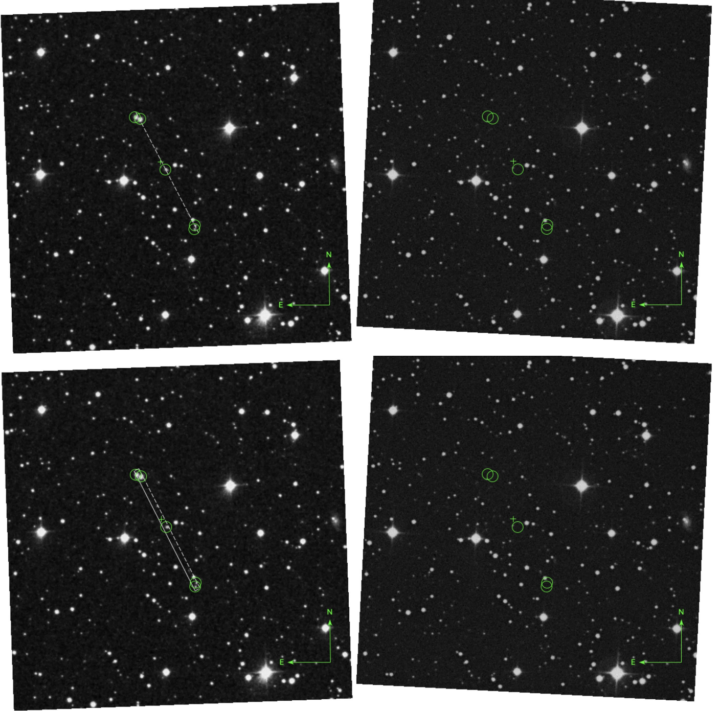
Figure 12. Candidate 5. We show the candidate in SuperCosmos scans of POSS-I red (left) and POSS-II red (right) images. The upper row shows a 3-point alignment within 1 arcsec. The lower row shows a 5-point alignment of within 10 arcsec. Transients are marked with green circles. The candidate with a measured coordinate is marked with a cross (+). The dashed lines shows the alignment (the white double line for the thicker alignment below).
