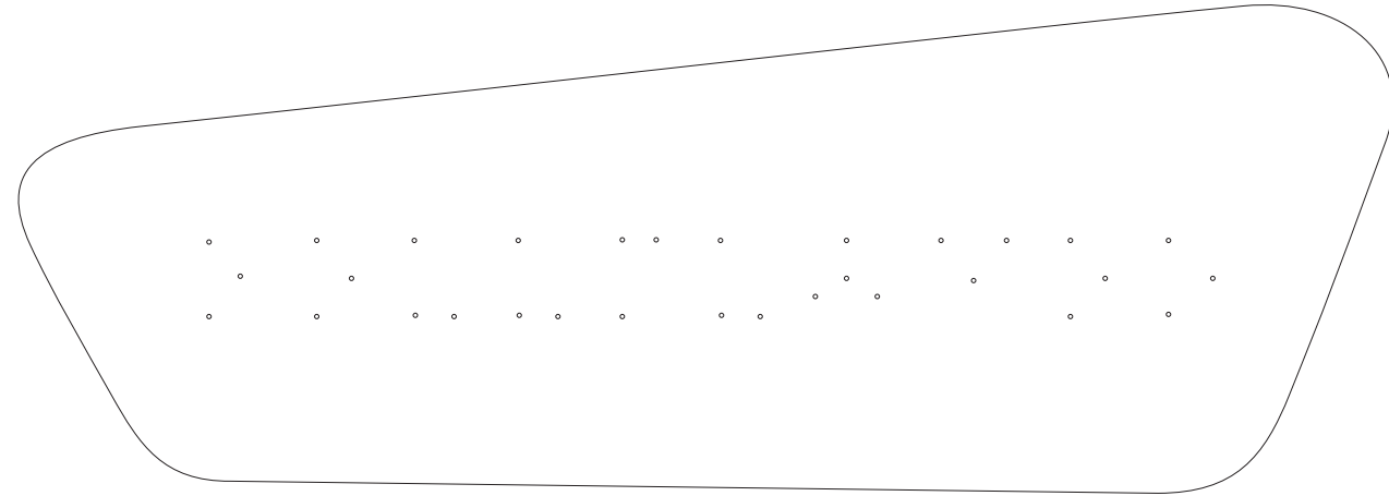
Stud Pattern for Letters - Front of Pan A sand texture finish removed for visibility
