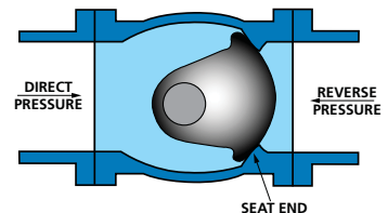
Figure 5. Installation Orientation
