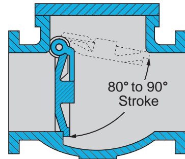
Figure 2. Conventional Swing Check Valve
