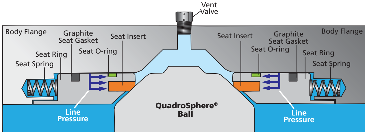
Figure 3 - Bi-directional Sealing
