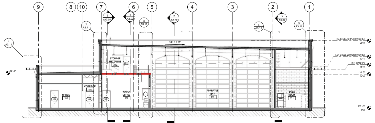
1 BUILDING SECTION 1/8" = 1'-0"
