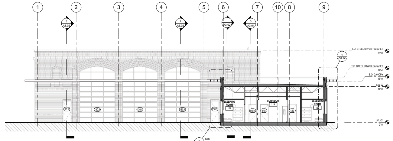
2 BUILDING SECTION 1/8" = 1'-0"
