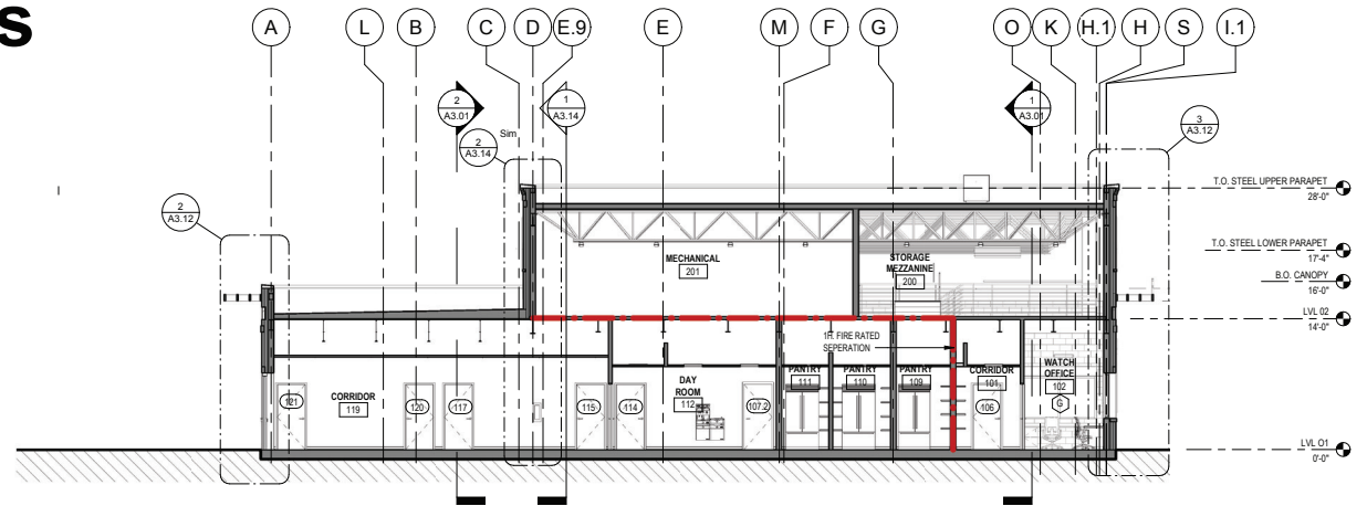
3 BUILDING SECTION 1/8" = 1'-0"
