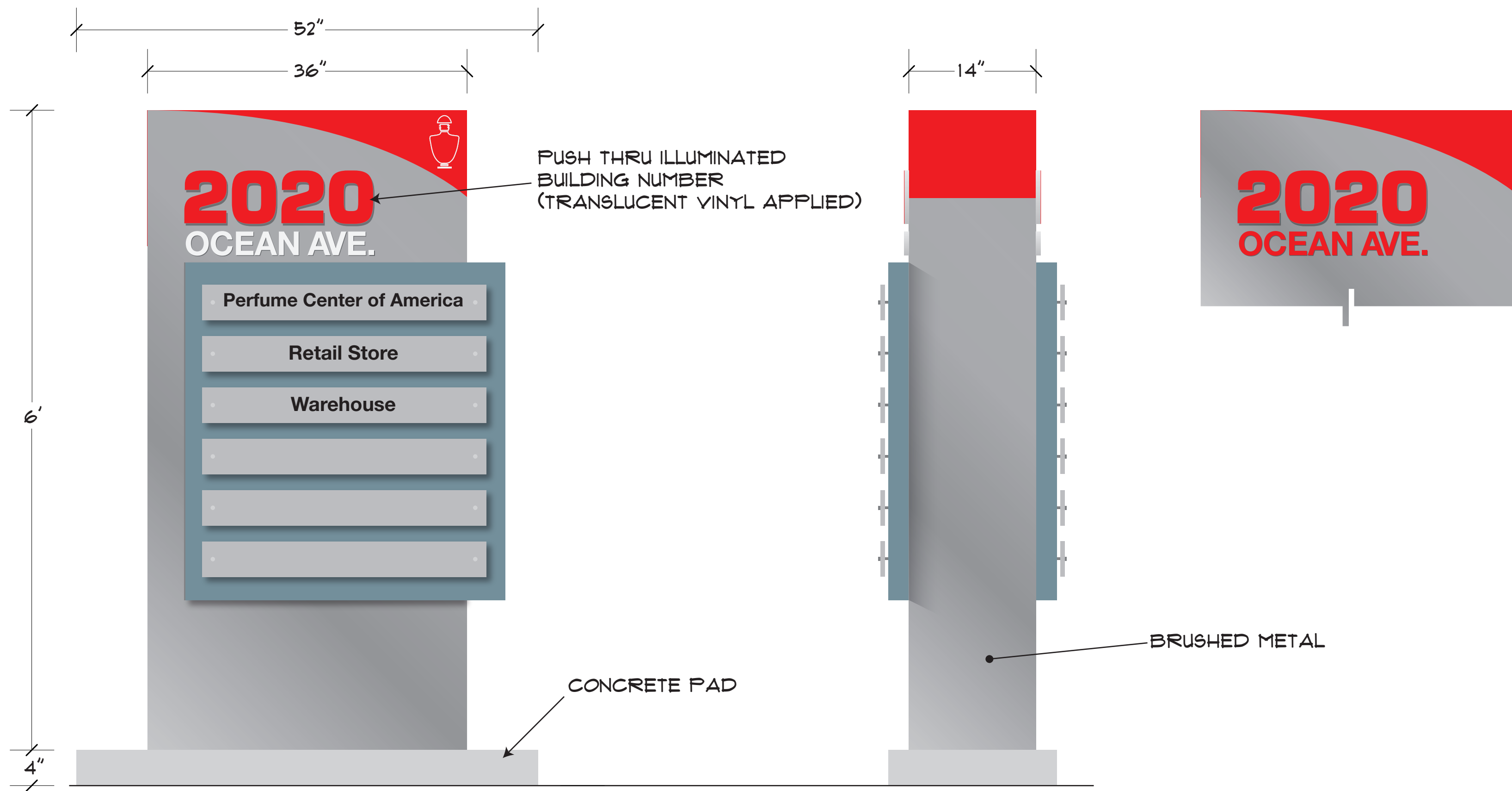
1 D/F INTERNALLY ILLUMINATED MONUMENT SIGN SCALE: NTS
