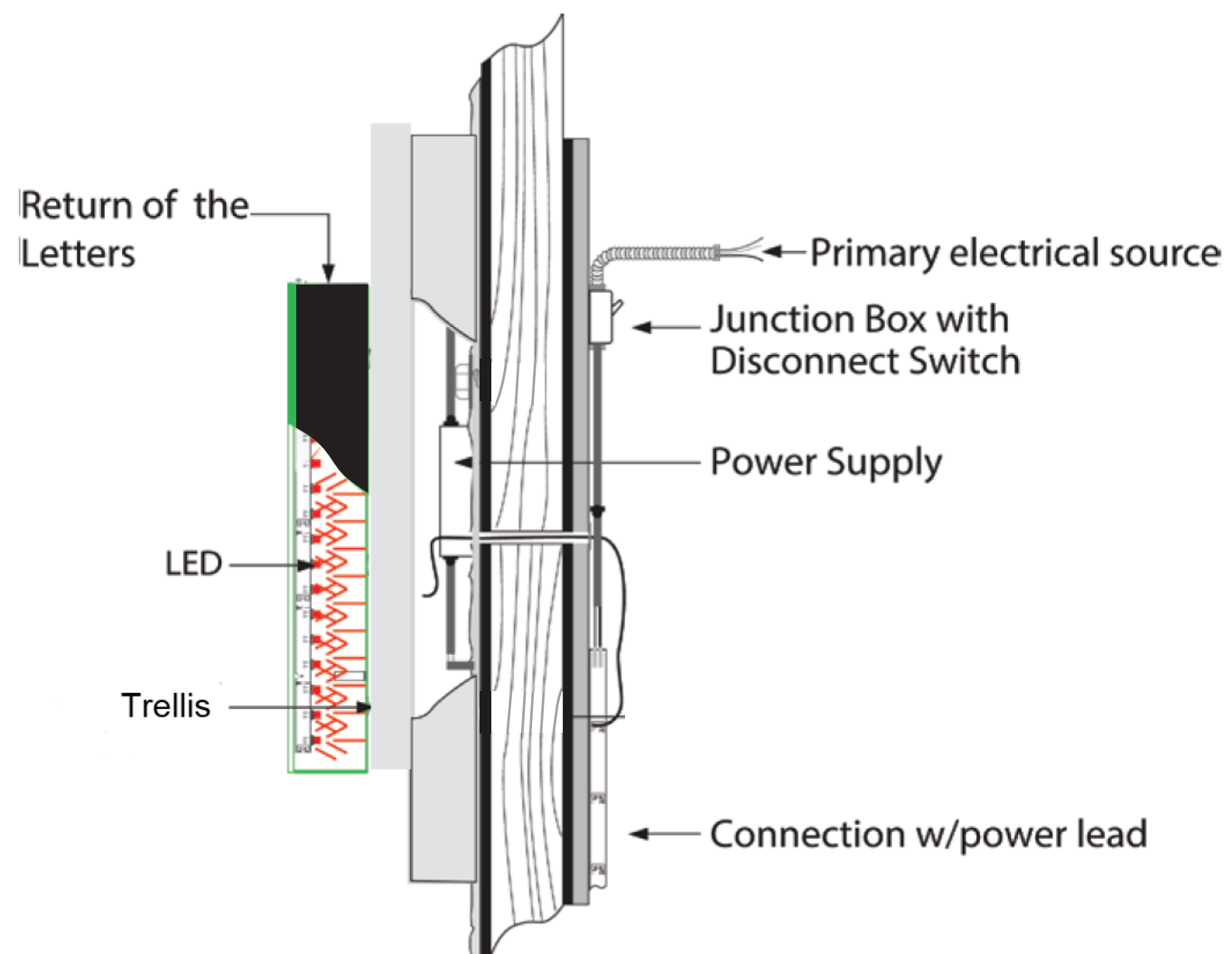
2 SIDE VIEW / FLUSH MOUNT CROSS SECTION SCALE = NTS
