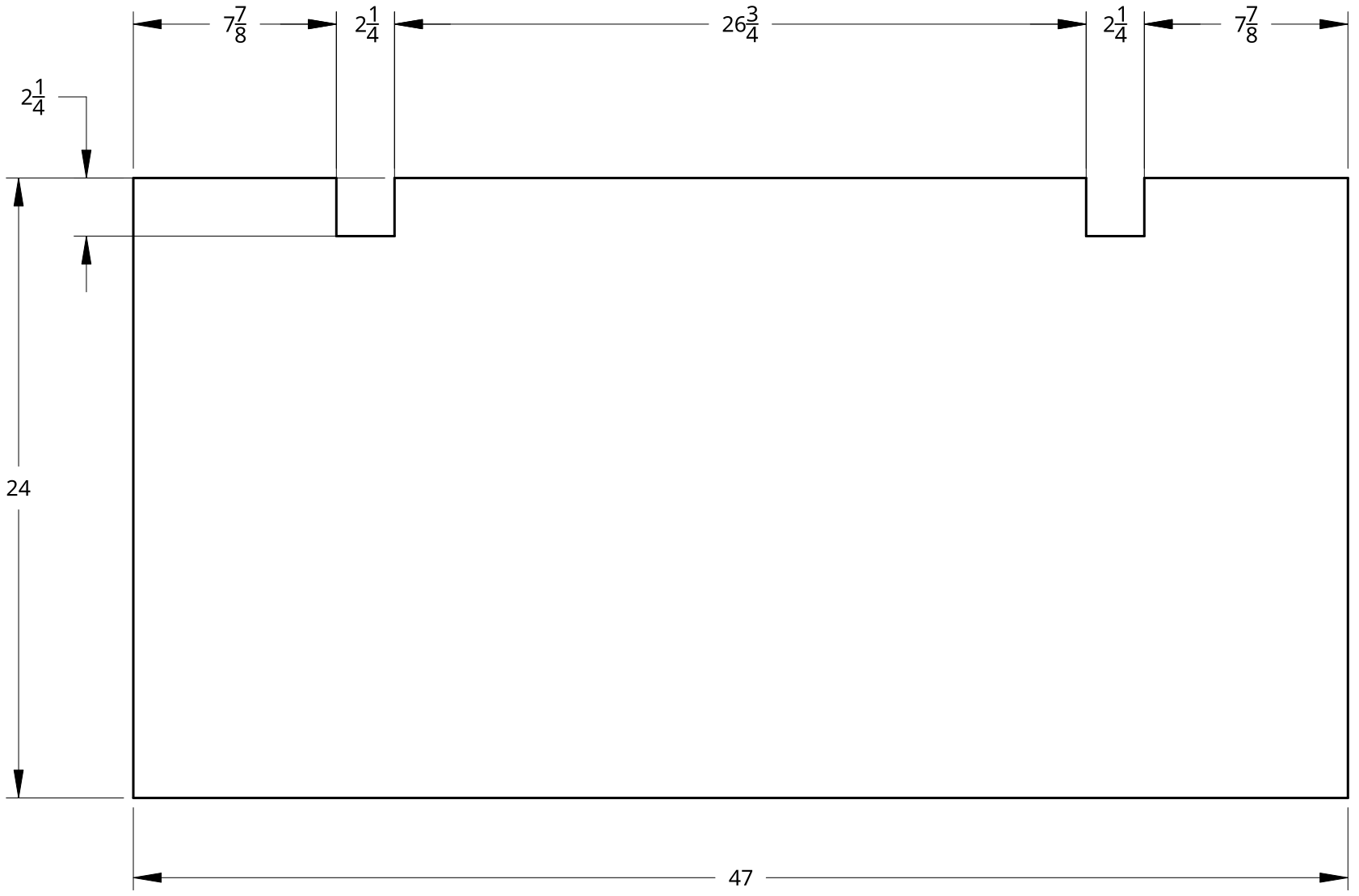
PL-07 - Platform Top
