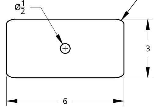
TRF-05 - Chute Support Arm Cap
