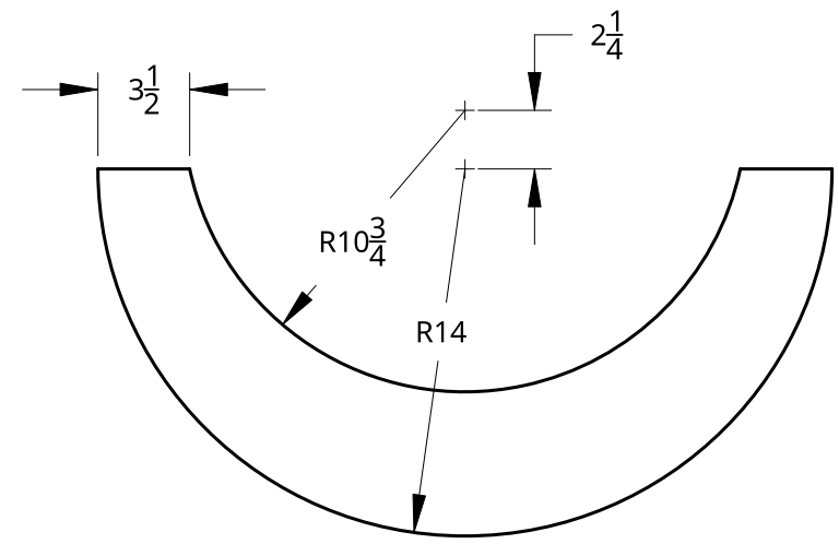
TRF-01
