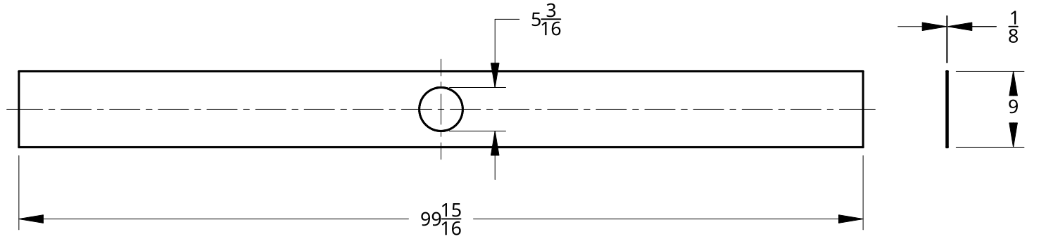
TRR-02
