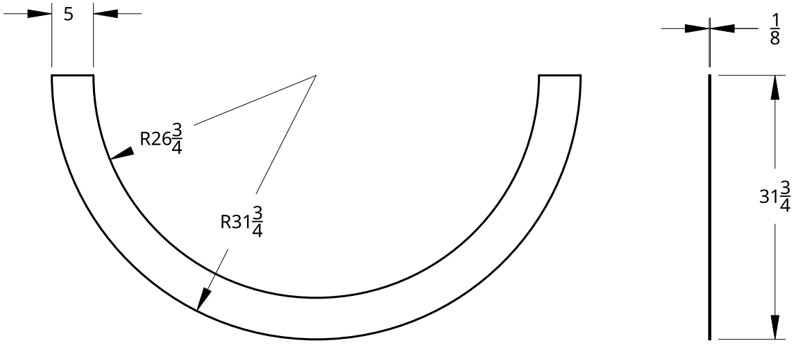
TRR-03
