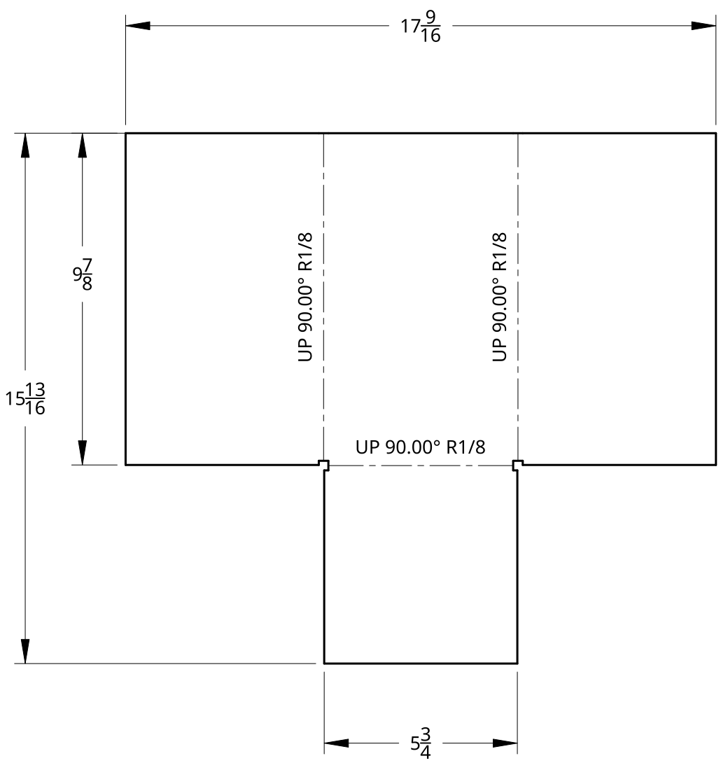
CB-01 CONTROL BOX
