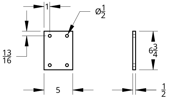
CS-04 - Caster Support Plate
