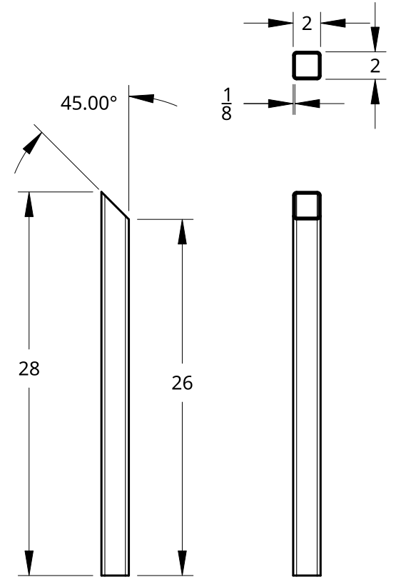
CS-01 - Front Caster Support Leg
