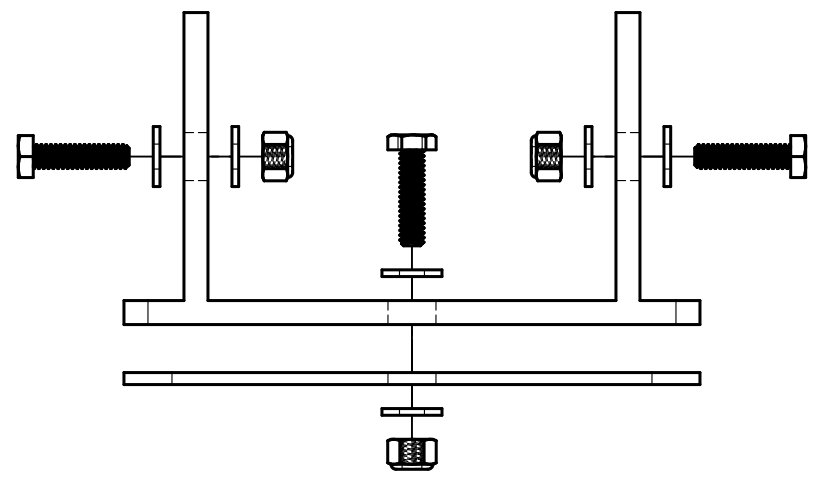
Chute Support Assembly
