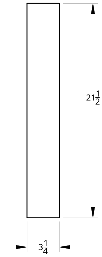
PL-06 - Platform Step (Rolled and spot welded to Step Flange)
