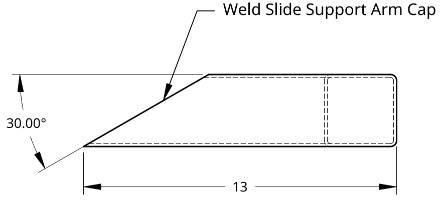
TRF-04 - Chute Support Arm
