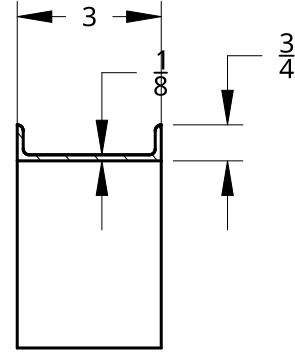
SECTION A - A SCALE 1:4
