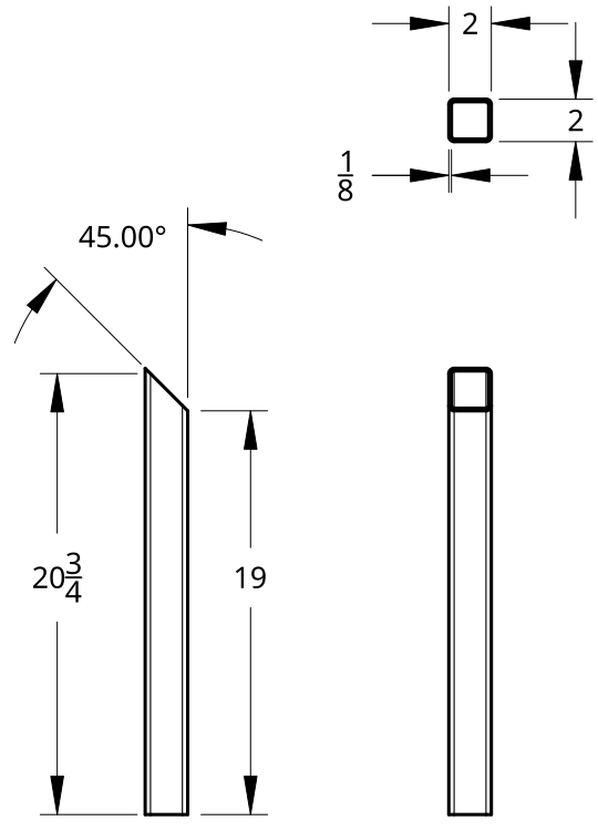
CS-02 - Rear Caster Support Leg
