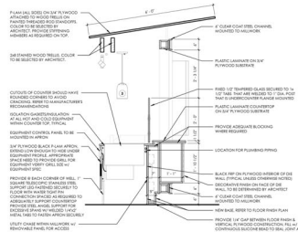
3 HEALTH & WELLNESS SECTION 1/4" = 1'-0"
