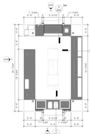
1 ENLARGED PLAN - HEALTH & WELLNESS 1/4" = 1'-0"
