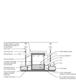
4 HEALTH & WELLNESS 1 1/4" = 1'-0"
