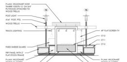
6 HEALTH & WELLNESS 3 1/4" = 1'-0"
