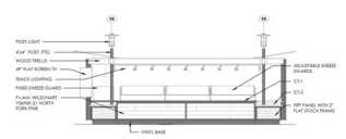
5 HEALTH & WELLNESS 2 1/4" = 1'-0"
