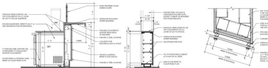
5 CAFE SECTION B 1/4" = 1'-0"
