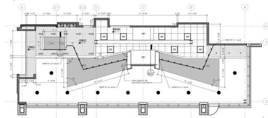
2 LEVEL 1 - RCP DETAIL - CAFE 1/4" = 1'-0"
