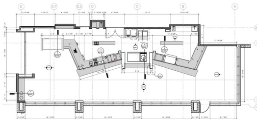
1 LEVEL 1 - ENLARGED PLAN - CAFE 1/4" = 1'-0"
