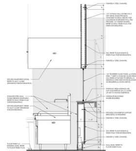
8 CAFE SECTION C 1/4" = 1'-0"
