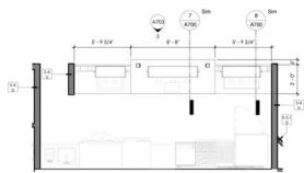
1 ENLARGED PLAN - SIMPLE SERVING 1/4" = 1'-0"
