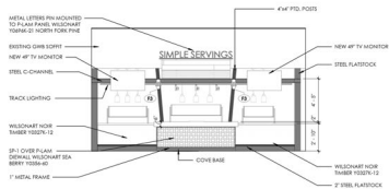
3 SIMPLE SERVING 1 1/4" = 1'-0"
