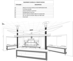
3 U CREATE 3D VIEW
