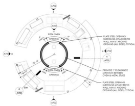
1 ENLARGED PLAN - PIZZA & PASTA 1/4" = 1'-0"
