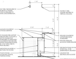
4 PIZZA & PASTA SECTION 1/4" = 1'-0"
