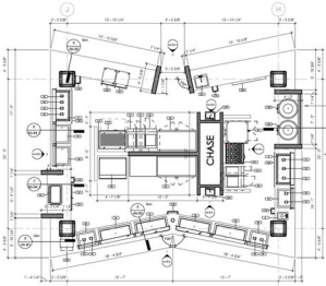
1 LEVEL 2 - ENLARGED PLAN - ISLAND STATION TWO
