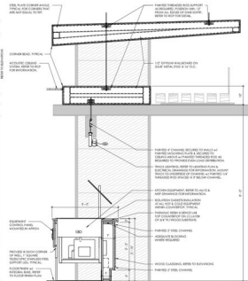
6 GRILL SECTION B
