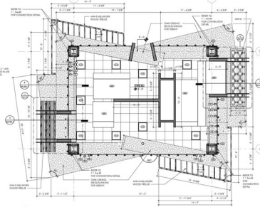
2 LEVEL 2 - RCP - ISLAND STATION TWO
