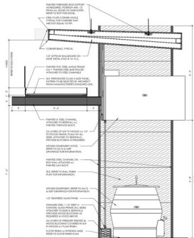
7 NAAN SECTION A
