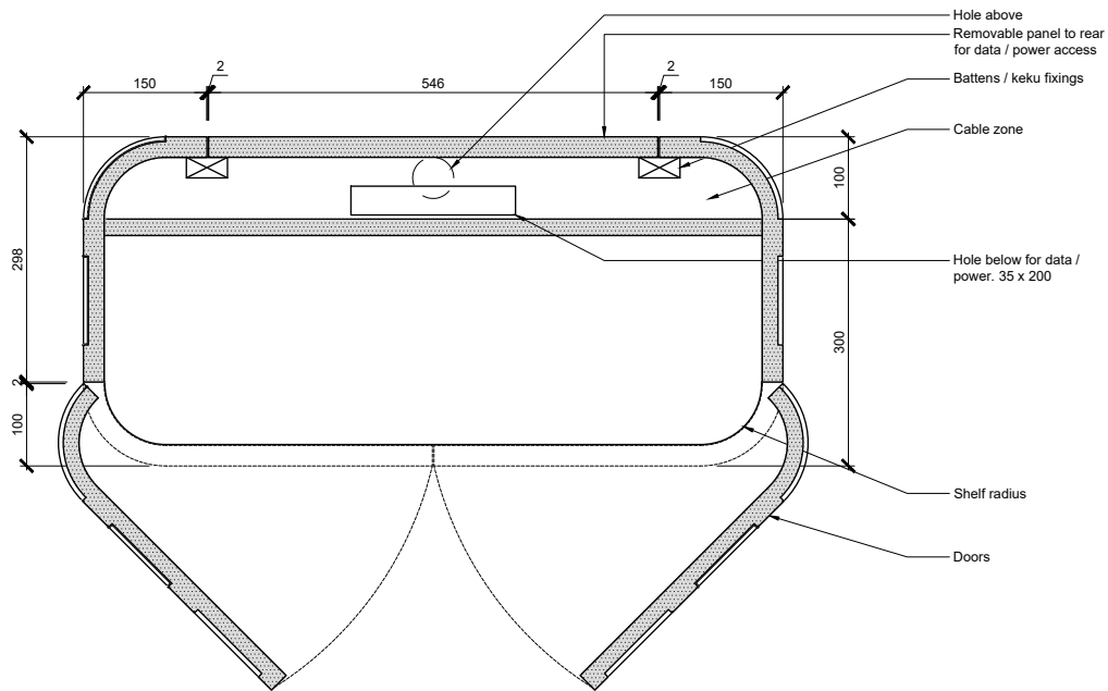
02 PLAN (LOW LEVEL)
