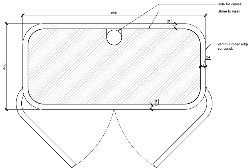
03 PLAN (HIGH LEVEL)
