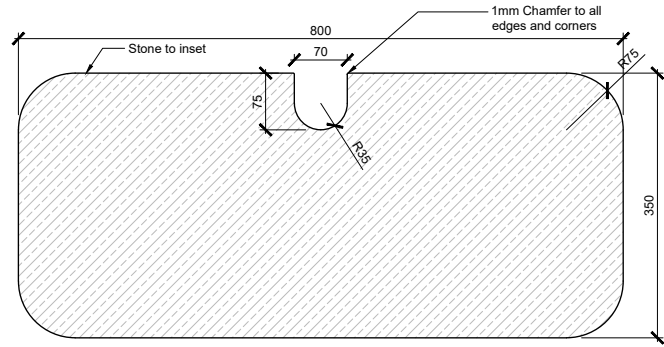
06 PLAN (Marble inset)
