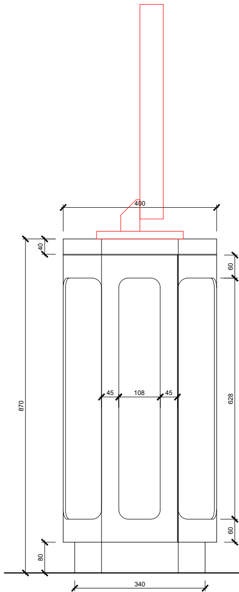
04 ELEVATION - SIDE
