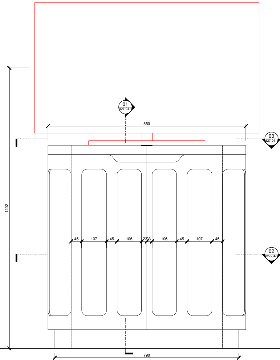
05 ELEVATION - FRONT
