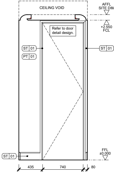
04 ELEVATION C scale 1:40 @A3 scale 1:20 @A1
