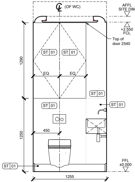
02 ELEVATION A scale 1:40 @A3 scale 1:20 @A1
