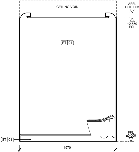
05 ELEVATION D scale 1:40 @A3 scale 1:20 @A1
