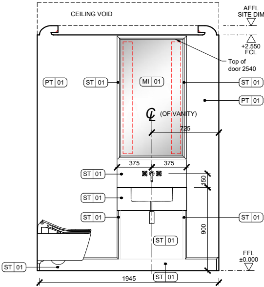
03 ELEVATION B scale 1:40 @A3 scale 1:20 @A1
