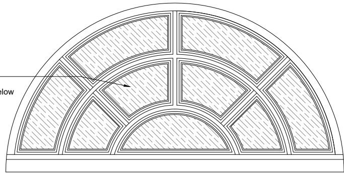
7 Elevation Detail, 1st Scale 1:5 Arched Window
