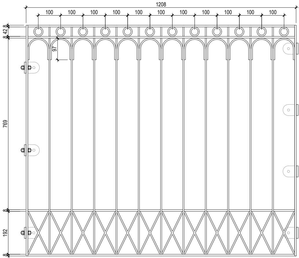
3 Detail, 1st Metal Balustrade Scale 1:5 Front Elevation
