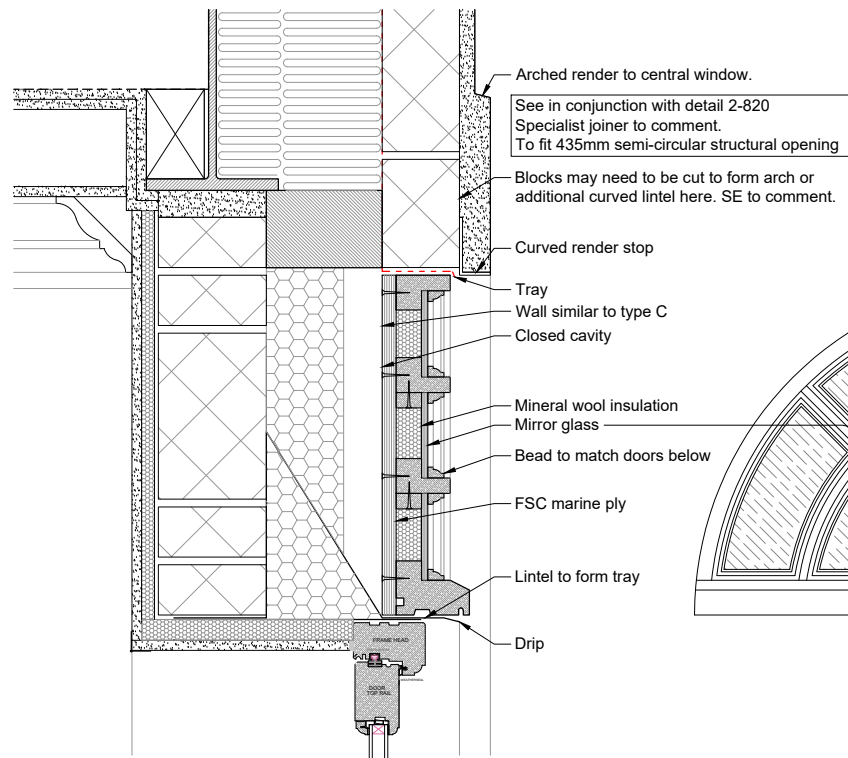
6 Section Detail, 1st Scale 1:5 Arched Window
