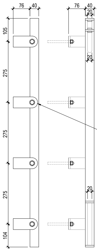
4 Detail, 1st Metal Balustrade Scale 1:5 Side Elevation
