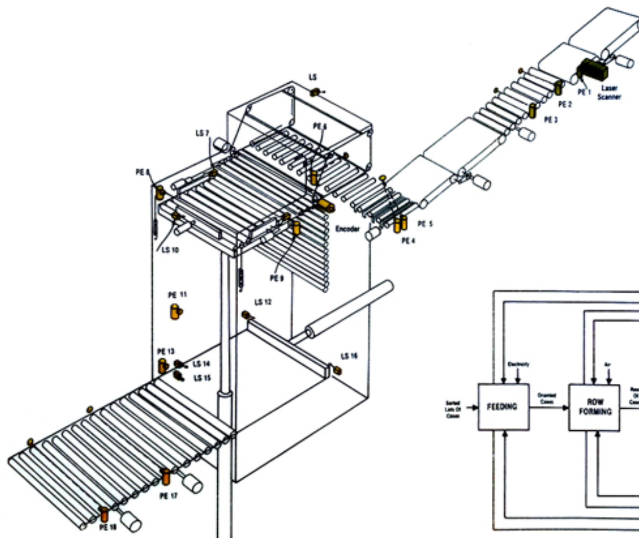
Controlling Function/Programmable Controller Input Devices
