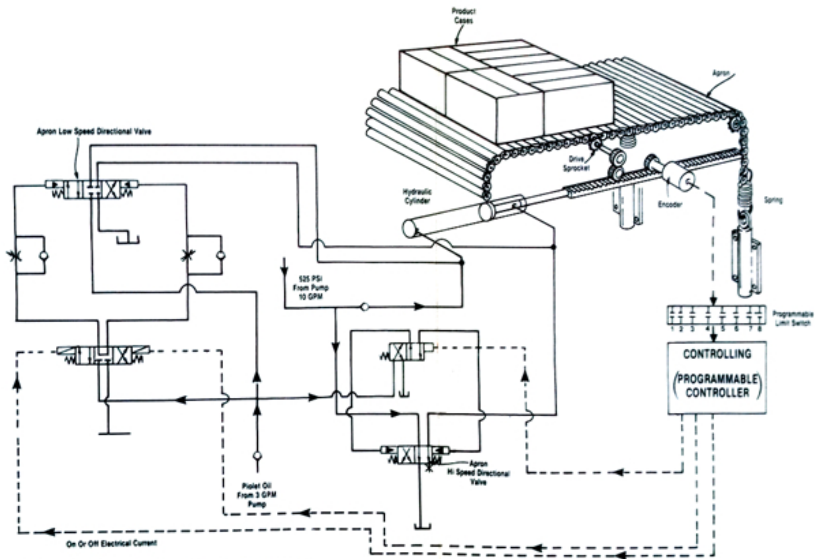
Fig. 11A1 Apron Machine Action Detail (Hydraulic)
