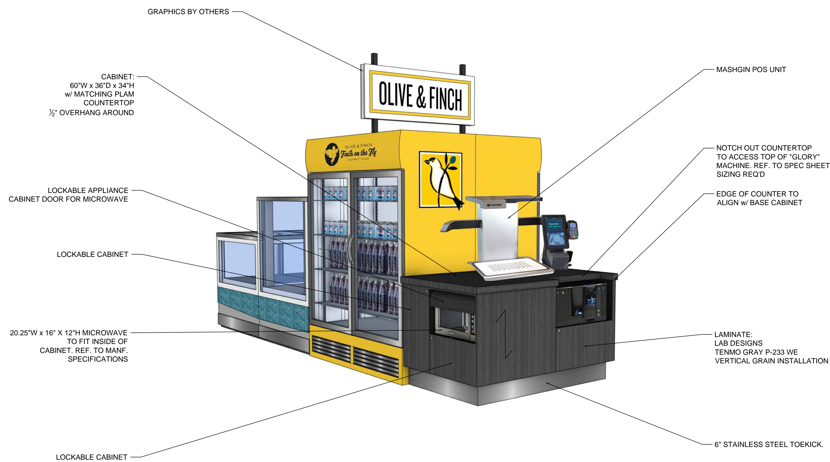
1 KIOSK - PERSPECTIVE 1/2" = 1'-0"
