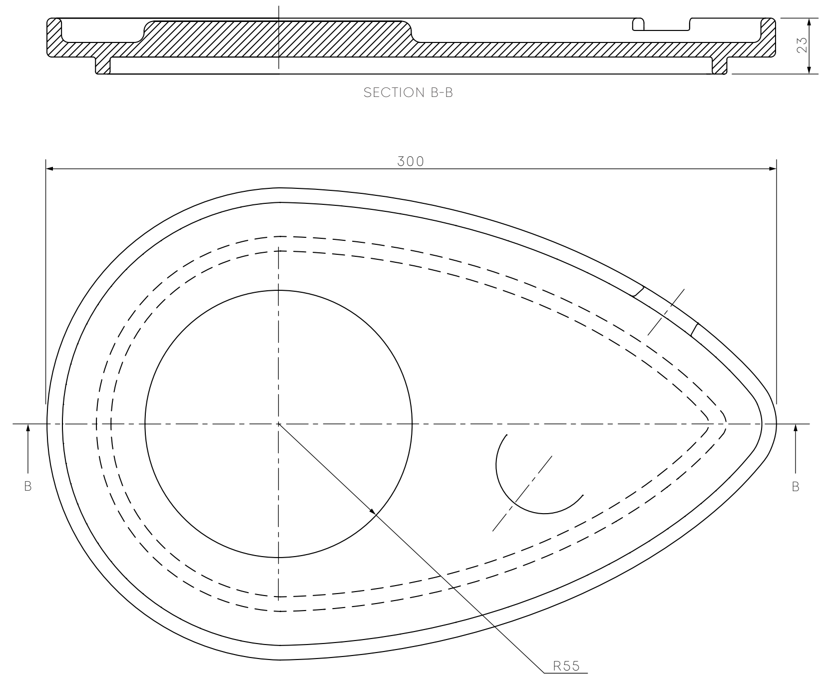
TECHNICAL DRAWINGS
