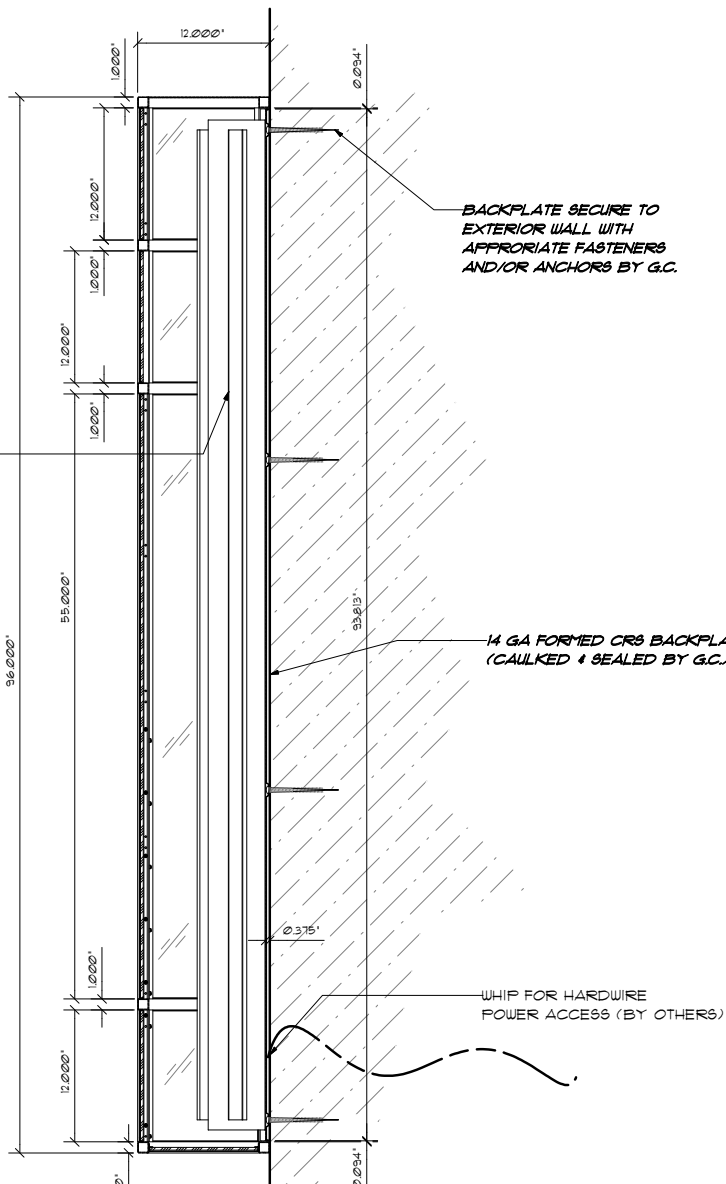
SECTION B-B SCALE 1/8
