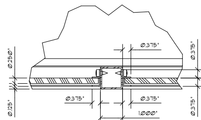
DETAIL P SCALE 1/2
