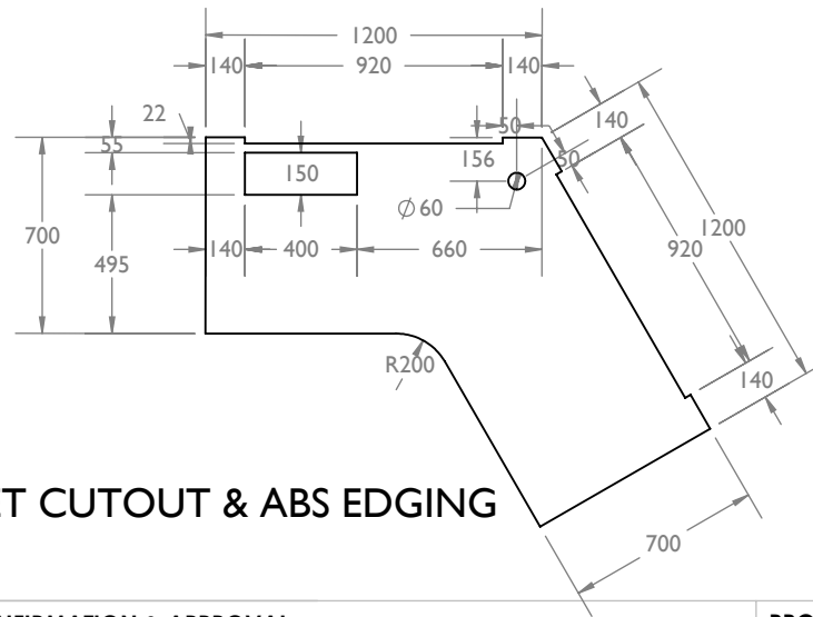
TRANS 20 PANEL
