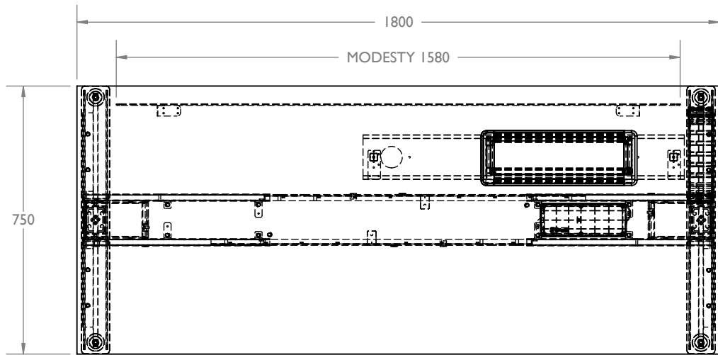
TOP VIEW
