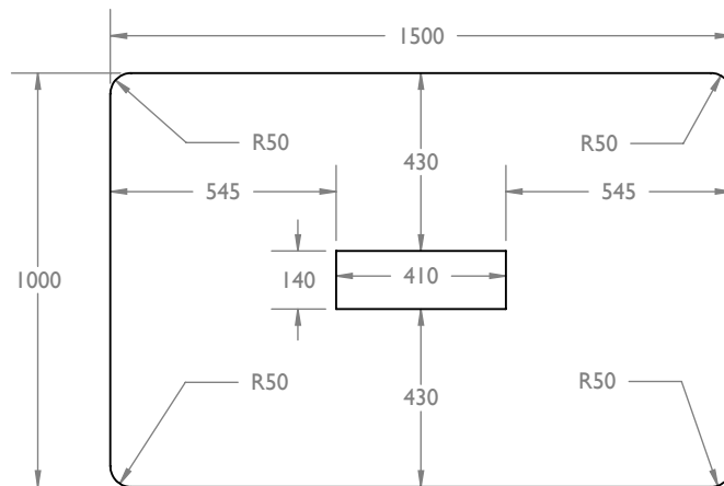
FLIPPER CUTOUT & ROUNDED CORNER
