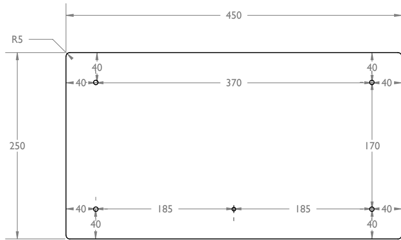
THICKNESS 4MM TOP PLATE CUTOUT VIEW
