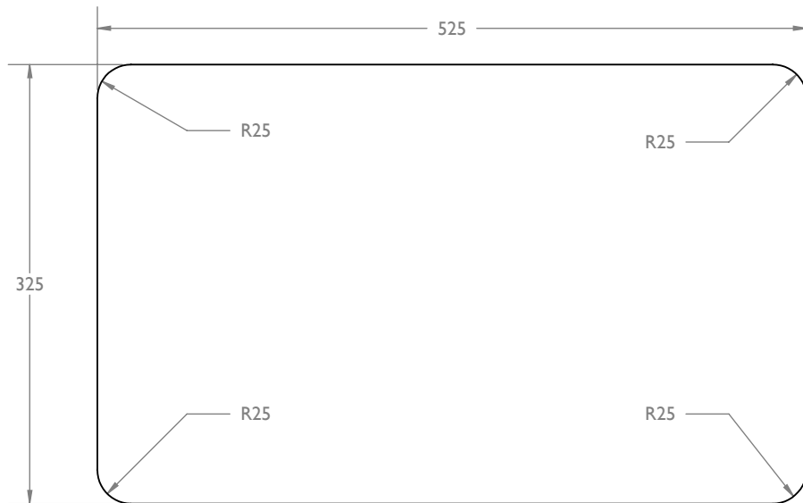
THICKNESS 9MM BOTTOM PLATE CUTOUT VIEW
