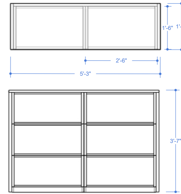
1 02 END-CAP TYPE B Scale: 1/2"=1'
