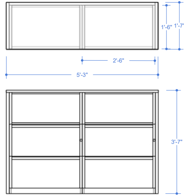
1 03 END-CAP TYPE C Scale: 1/2"=1'
