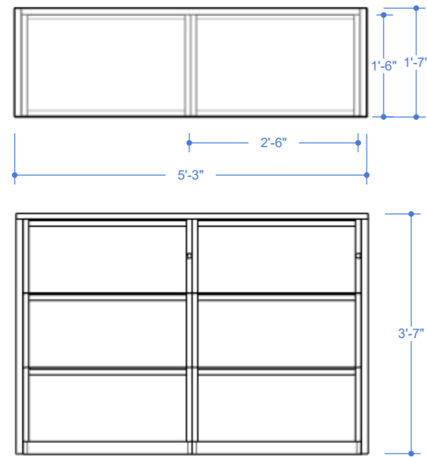
1 01 END-CAP TYPE A Scale: 1/2"=1'
