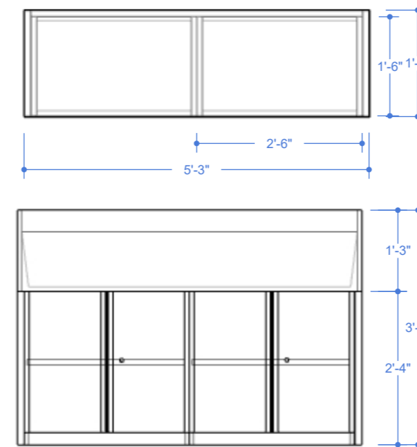
1 05 END-CAP TYPE F Scale: 1/2"=1'
