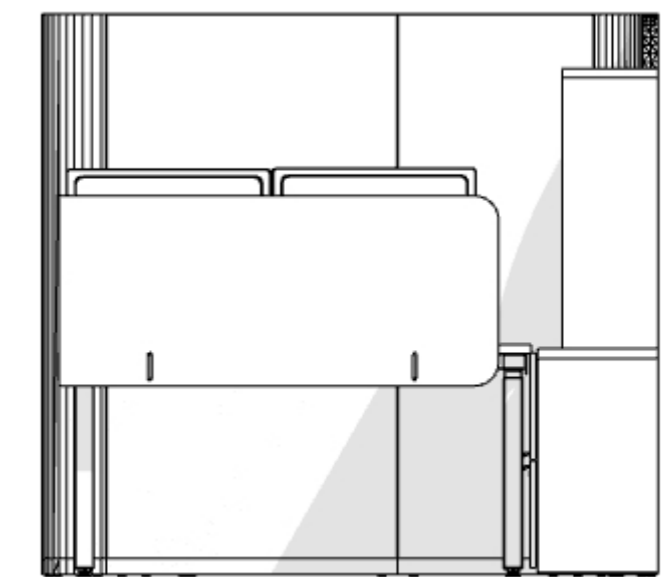
1 03 Elevation Scale: 1/4"=1'
