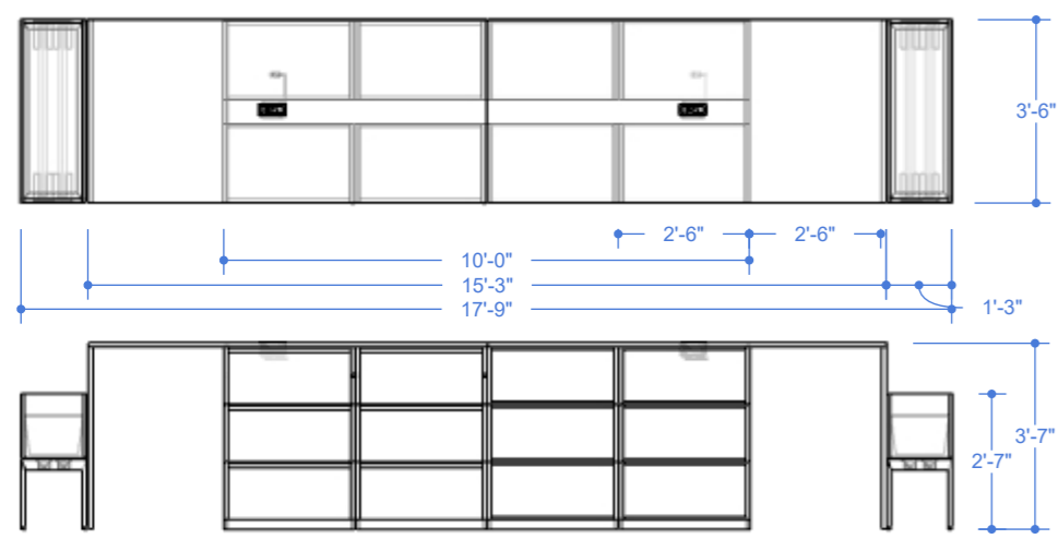
3 05 END-CAP TYPE E Scale: 1/4"=1'
