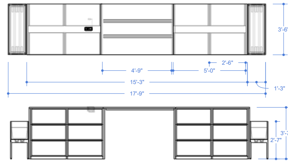
3 02 END-CAP TYPE B Scale: 1/4"=1'
