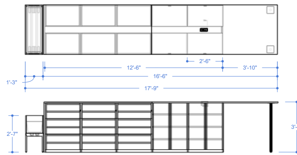
3 04 END-CAP TYPE D Scale: 1/4"=1'
