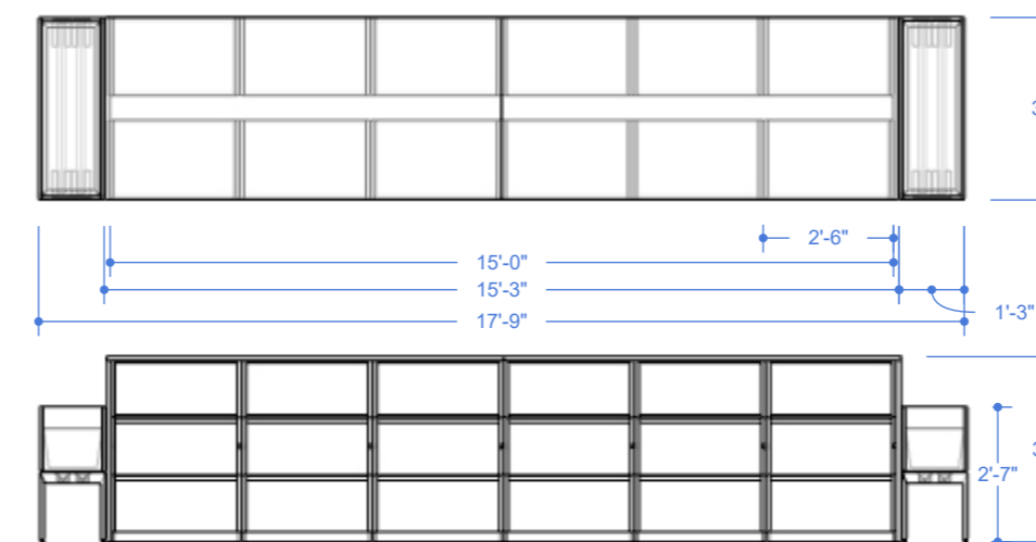
3 05 END-CAP TYPE F Scale: 1/4"=1'
