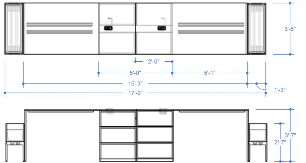
4 03 END-CAP TYPE C Scale: 1/4"=1'
