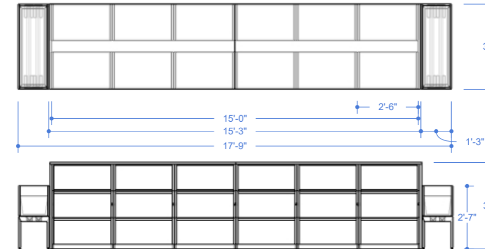
4 05 END-CAP TYPE F Scale: 1/4"=1'
